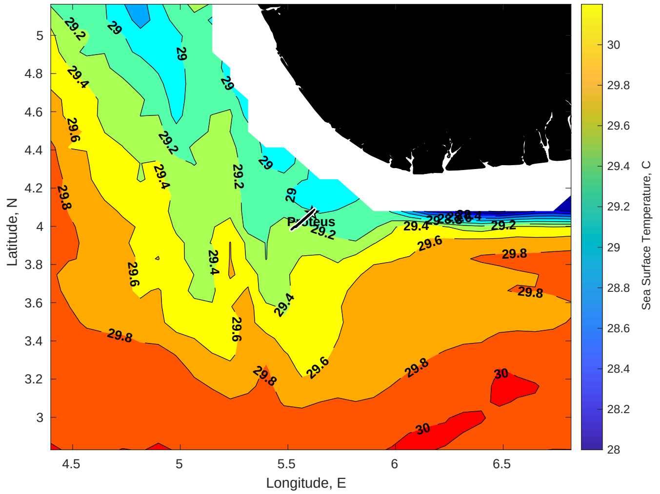
SST for Proteus at 07-Apr-2025 00:00:00
