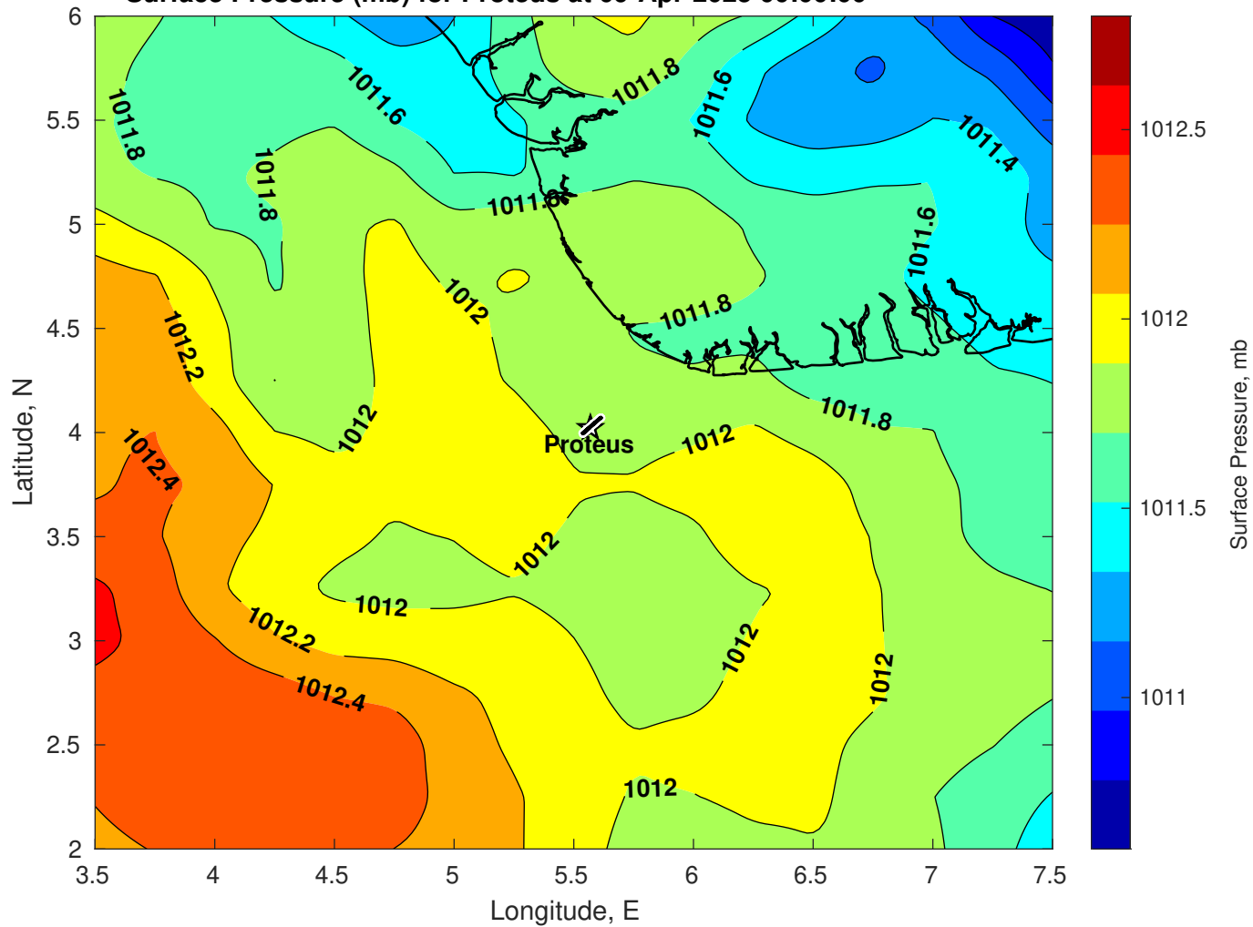
Surface Pressure (mb) for Proteus at 09-Apr-2025 00:00:00
