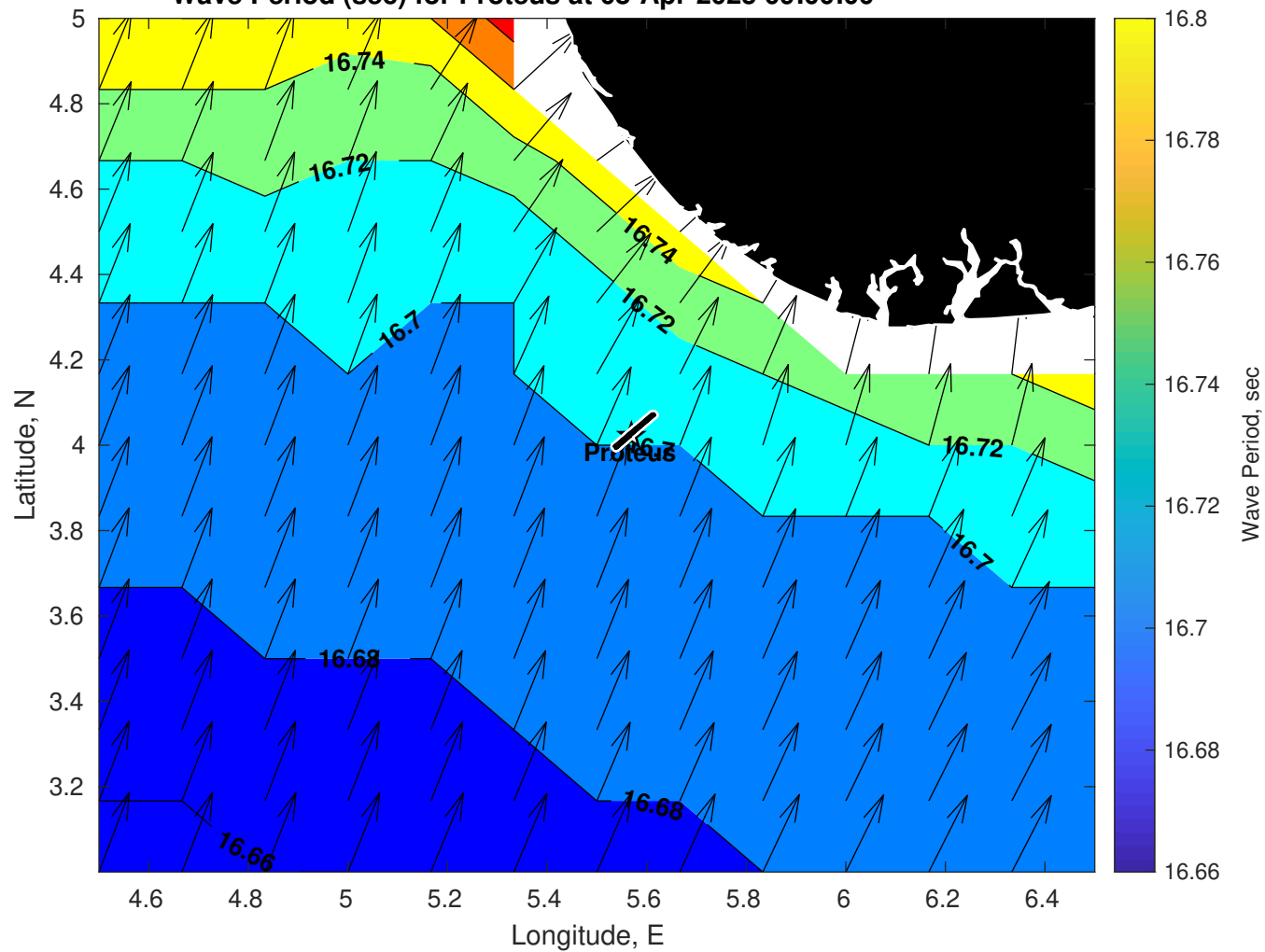
Wave Period (sec) for Proteus at 08-Apr-2025 09:00:00
