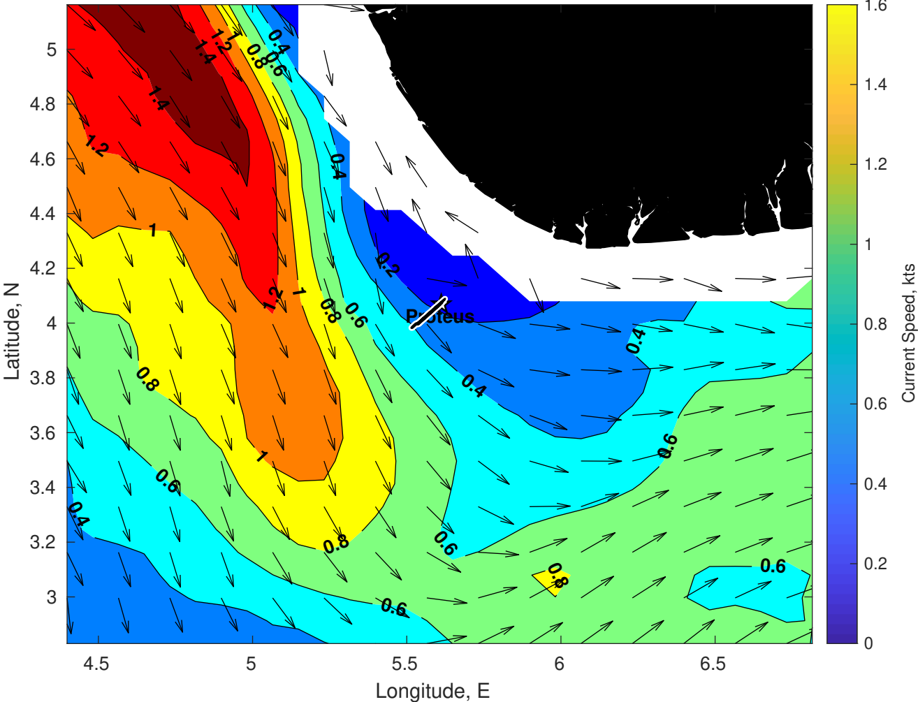
Surface Currents for Proteus at 07-Apr-2025 00:00:00
