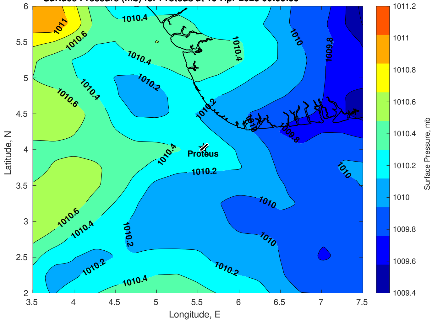
Surface Pressure (mb) for Proteus at 10-Apr-2025 00:00:00
