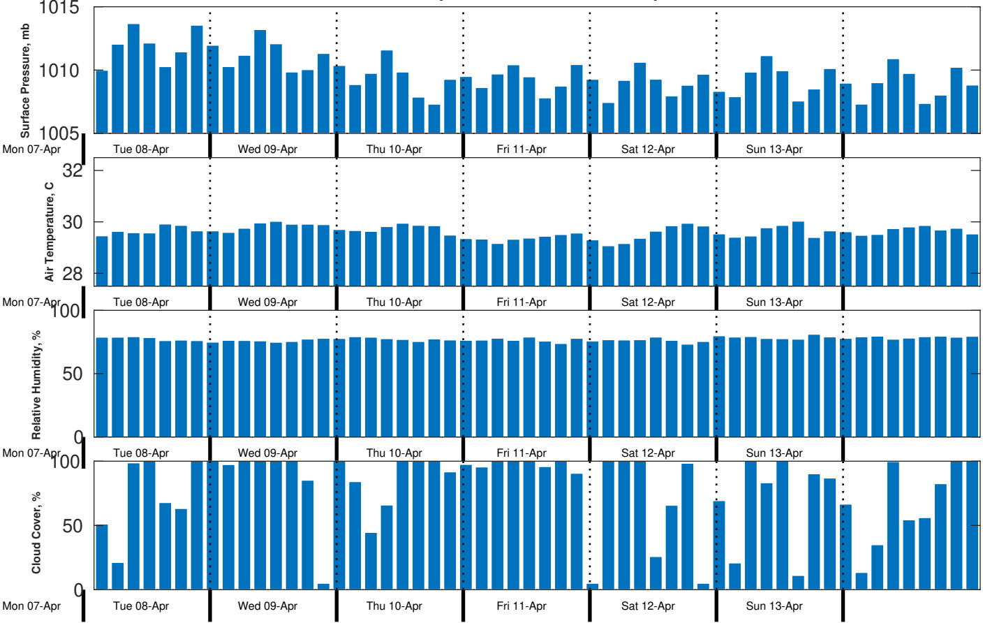
Met Forecast for Proteus from 08-Apr-2025 00:00:00 to 15-Apr-2025 00:00:00
