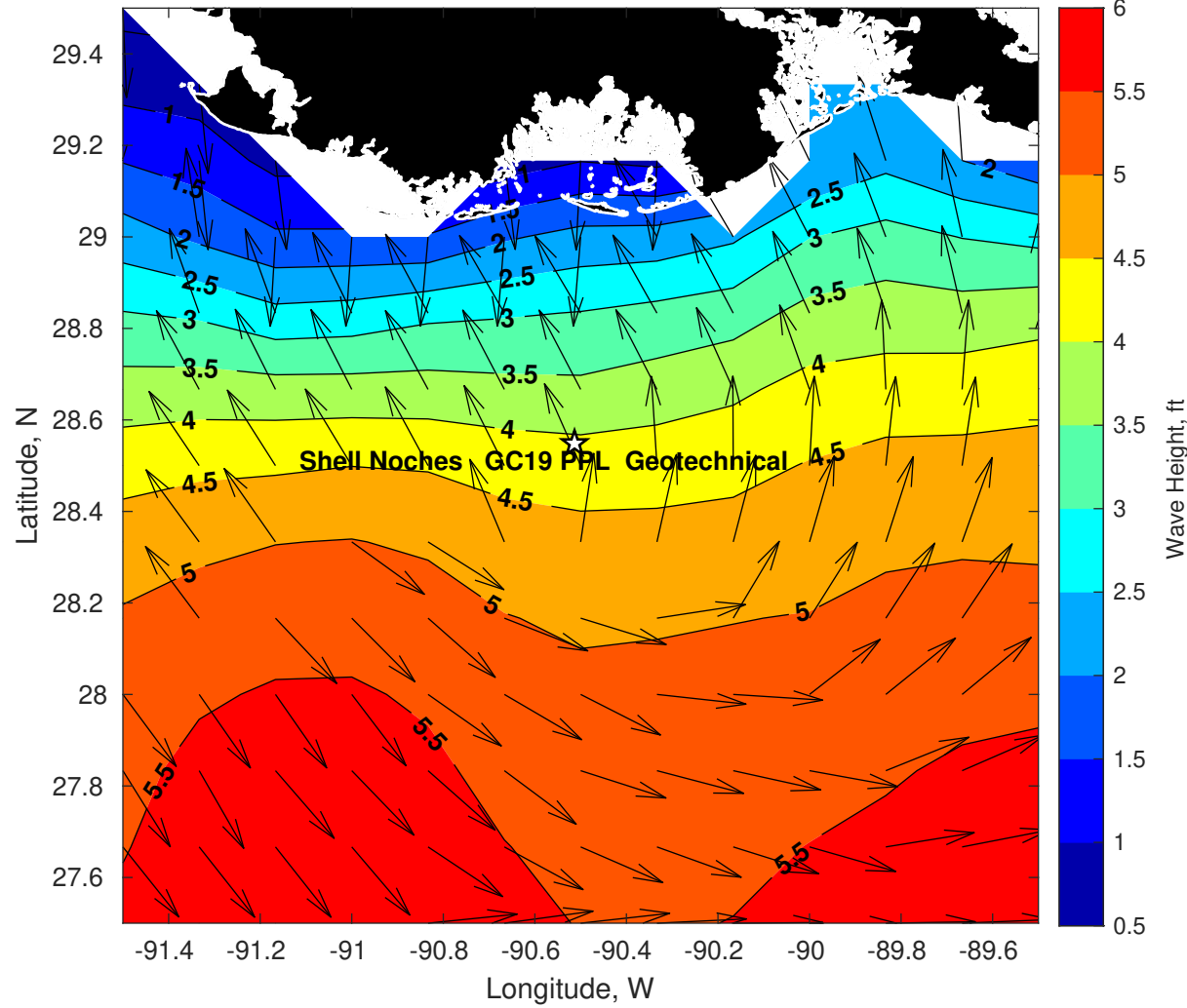
Wave Height (ft) for Shell Noches GC19 PPL Geotechnical at 08-Apr-2025 09:00:00
