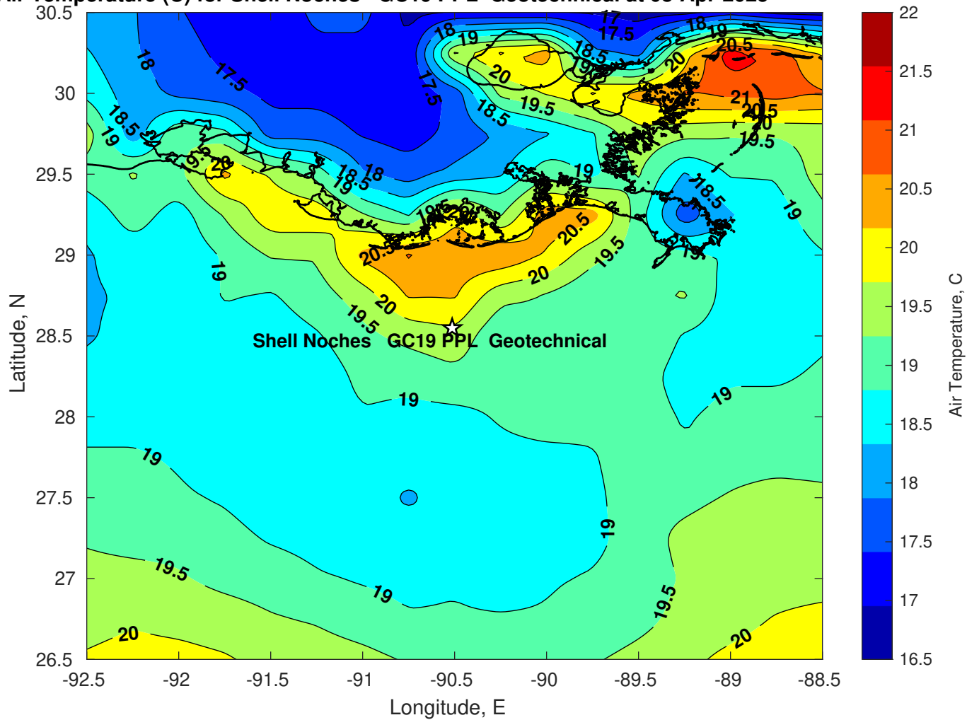
Air Temperature (C) for Shell Noches GC19 PPL Geotechnical at 08-Apr-2025
