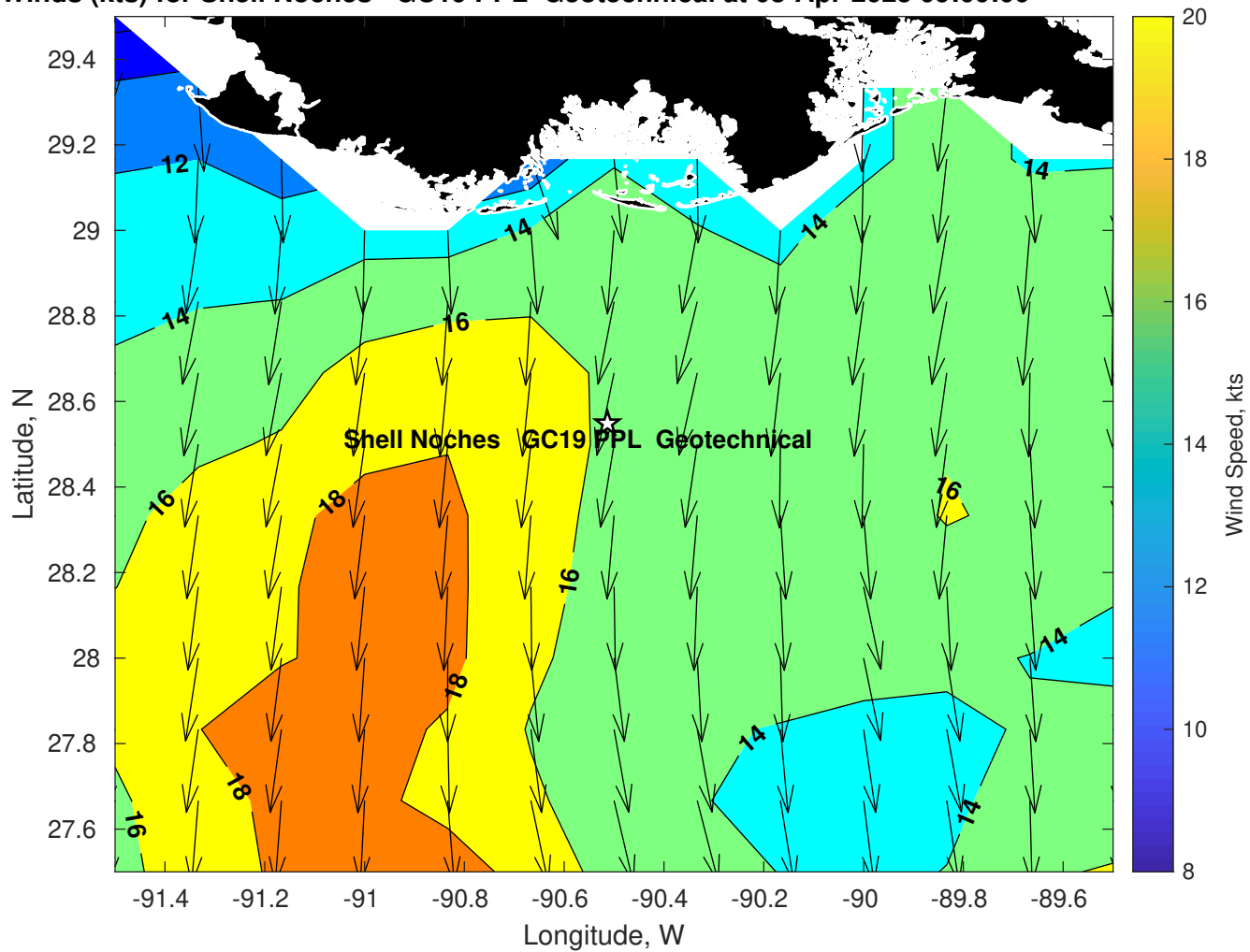
Winds (kts) for Shell Noches GC19 PPL Geotechnical at 08-Apr-2025 09:00:00
