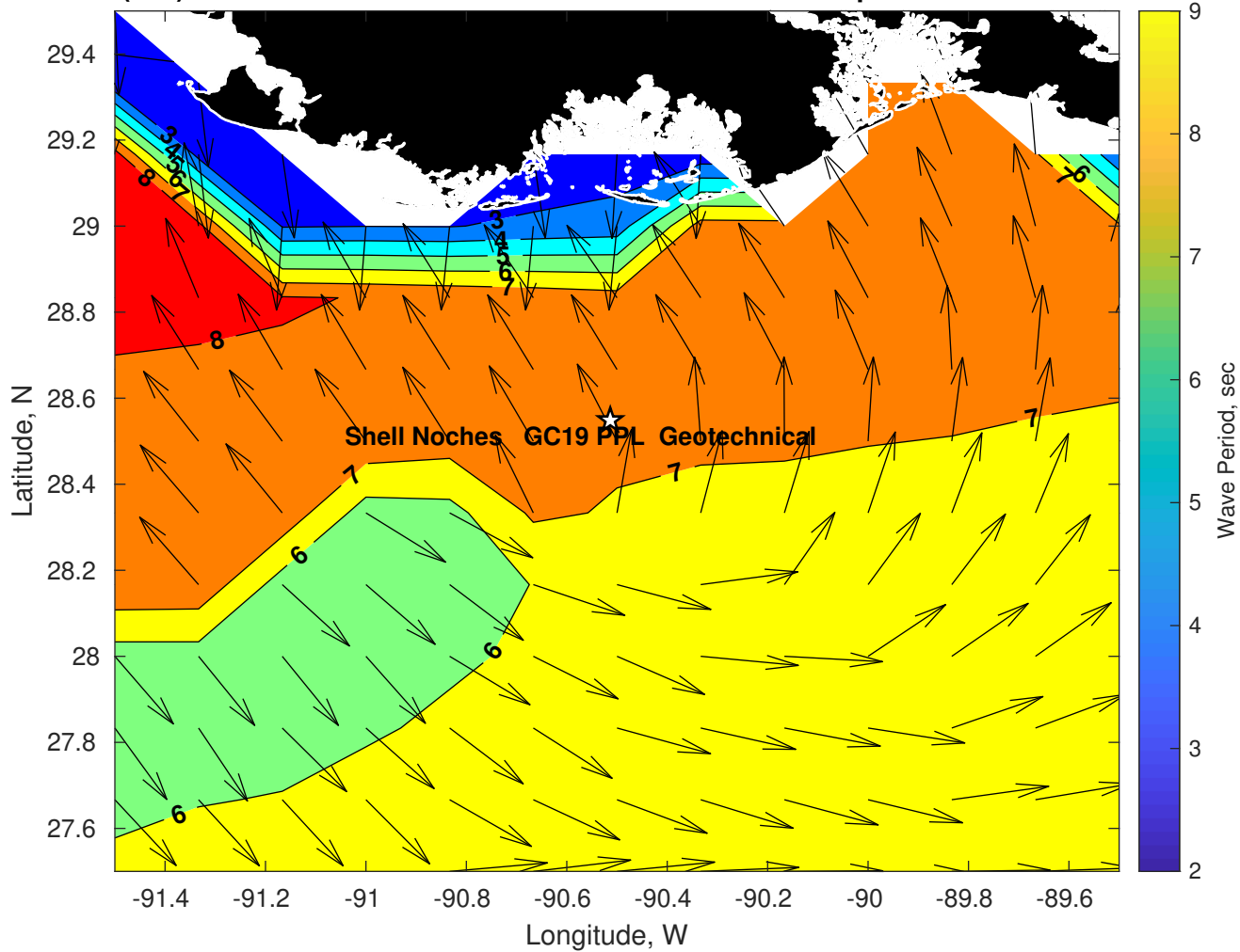
Wave Period (sec) for Shell Noches GC19 PPL Geotechnical at 08-Apr-2025 09:00:00
