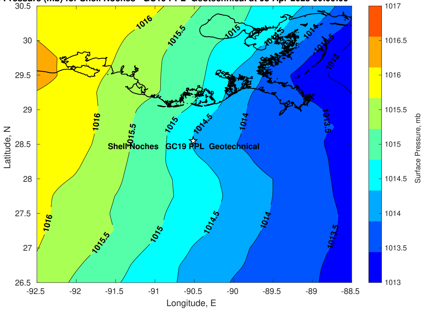
Surface Pressure (mb) for Shell Noches GC19 PPL Geotechnical at 08-Apr-2025 00:00:00
