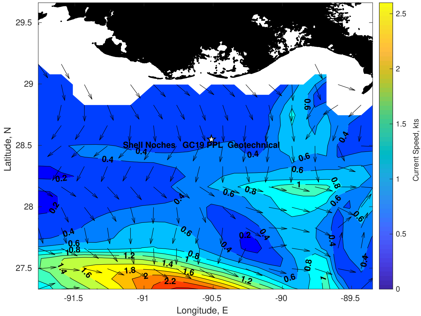
Surface Currents for Shell Noches GC19 PPL Geotechnical at 07-Apr-2025 00:00:00
