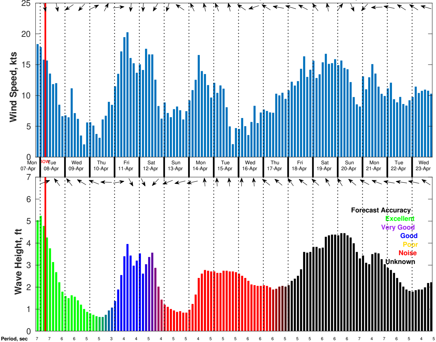
Wind & Wave Forecast for Shell Noches GC19 PPL Geotechnical from 07-Apr-2025 20:00:00 to 23-Apr-2025 20:00:00
