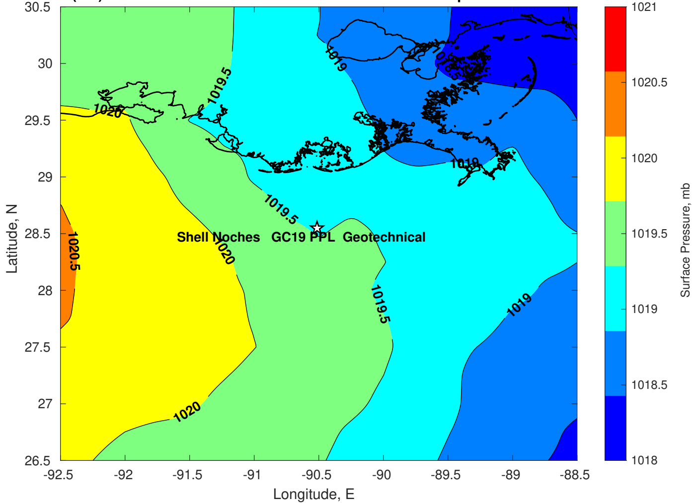
Surface Pressure (mb) for Shell Noches GC19 PPL Geotechnical at 09-Apr-2025 00:00:00
