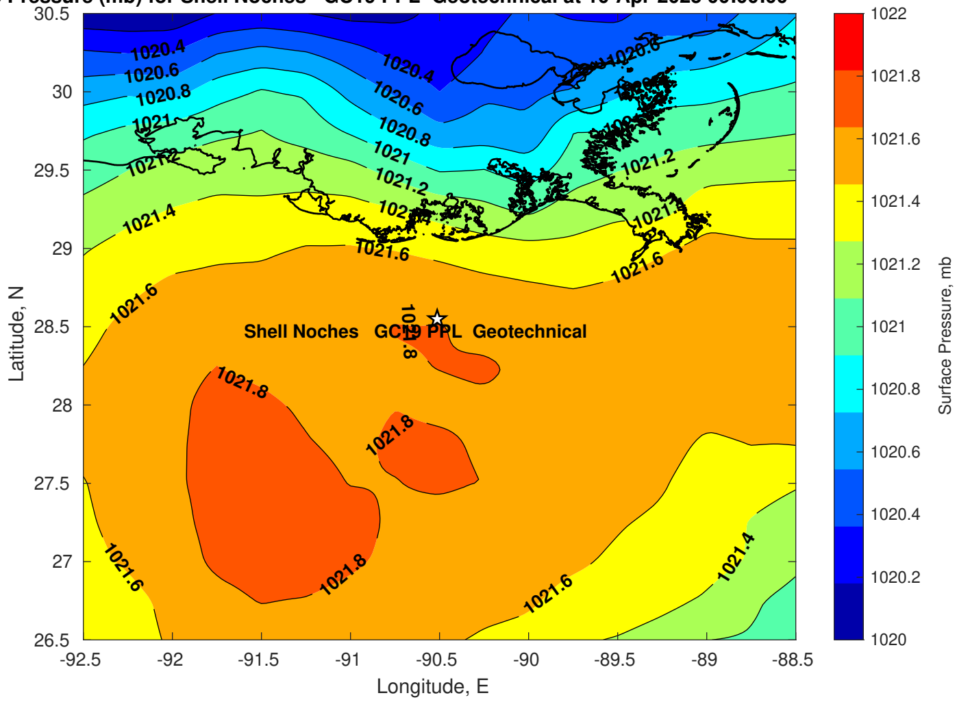
Surface Pressure (mb) for Shell Noches GC19 PPL Geotechnical at 10-Apr-2025 00:00:00
