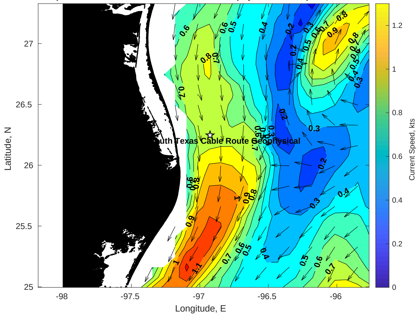
face Currents for Tampnet P2378 South Texas Cable Route Geophysical at 07-Apr-2025 00:00:00
