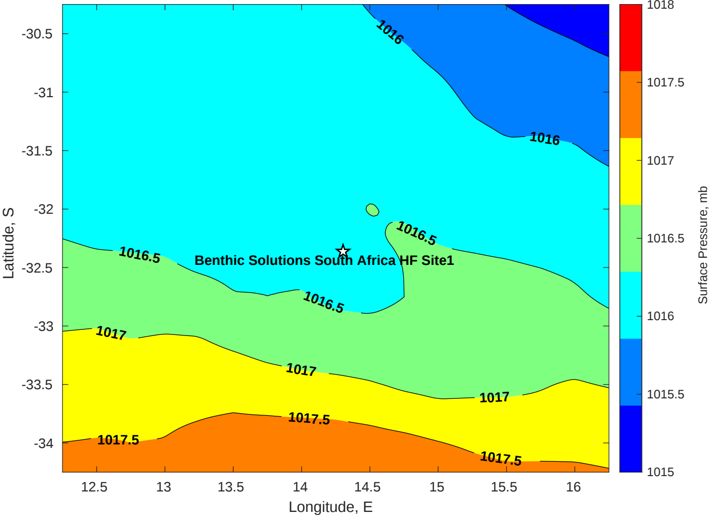
Surface Pressure (mb) for Benthic Solutions South Africa HF Site1 at 10-Apr-2025 00:00:00
