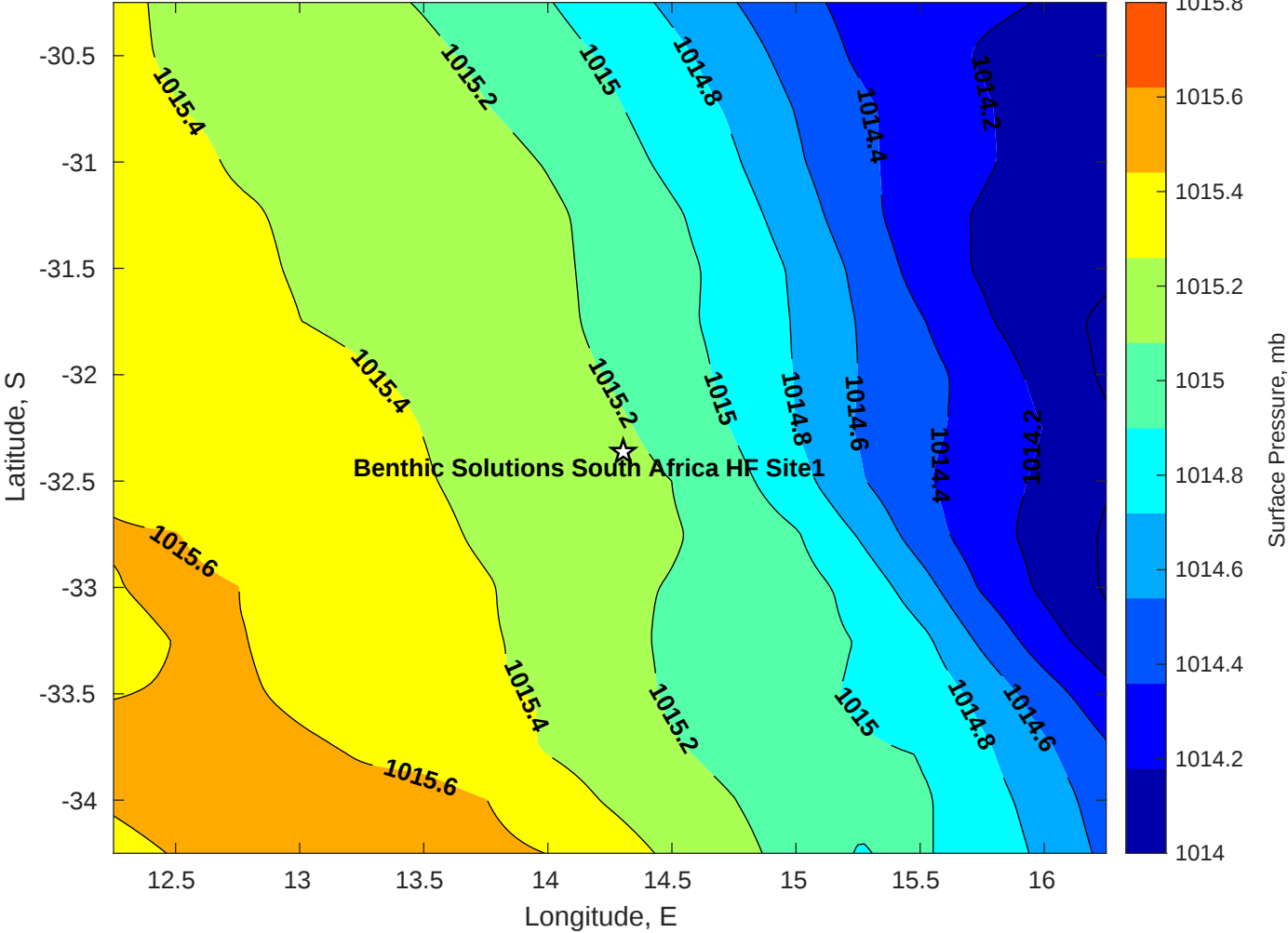
Surface Pressure (mb) for Benthic Solutions South Africa HF Site1 at 11-Apr-2025 00:00:00
