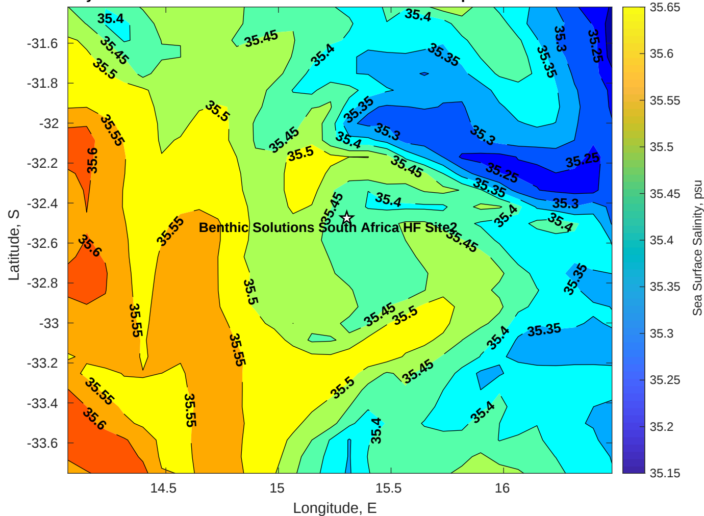
Surface Salinity for Benthic Solutions South Africa HF Site2 at 08-Apr-2025 00:00:00
