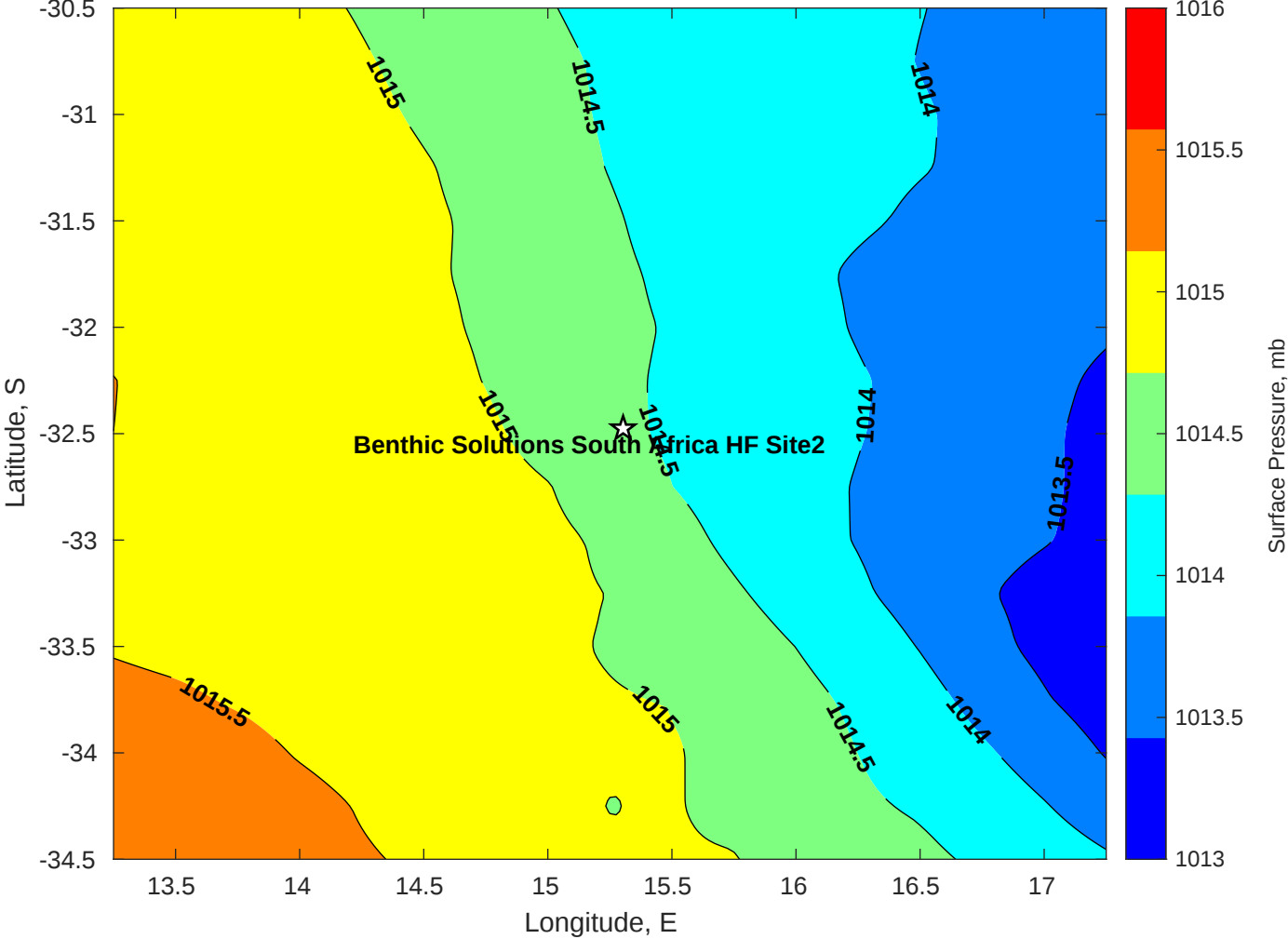
Surface Pressure (mb) for Benthic Solutions South Africa HF Site2 at 11-Apr-2025 00:00:00
