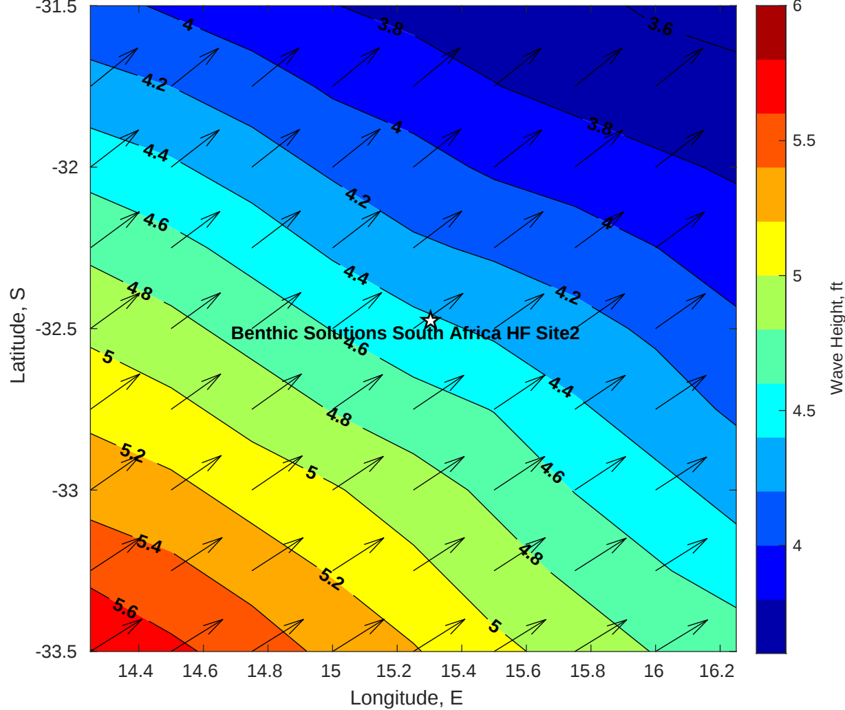
Wave Height (ft) for Benthic Solutions South Africa HF Site2 at 09-Apr-2025 09:00:00
