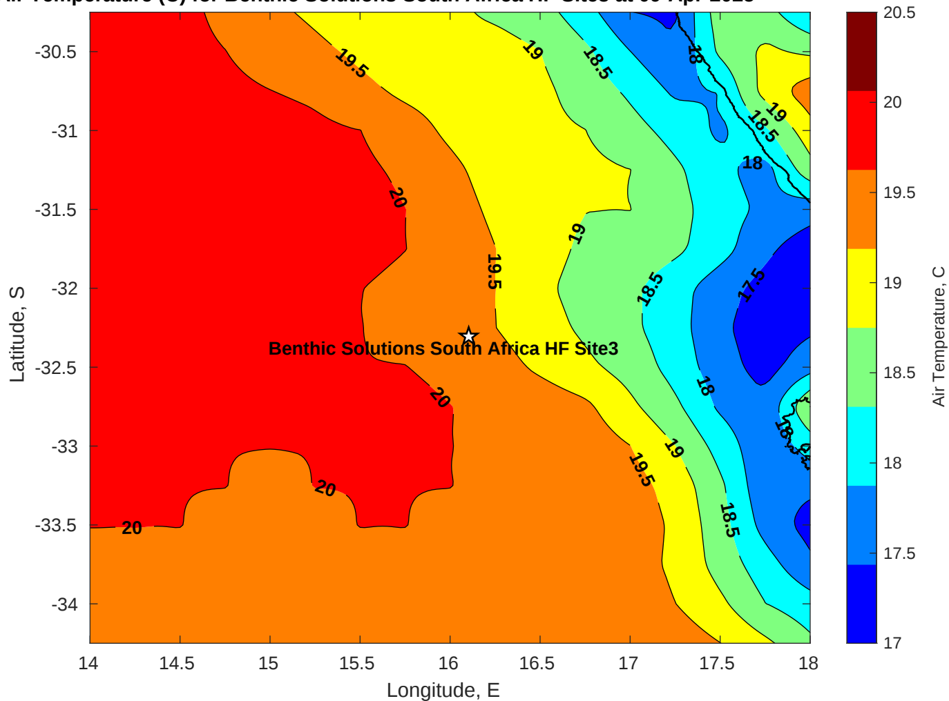
Air Temperature (C) for Benthic Solutions South Africa HF Site3 at 09-Apr-2025
