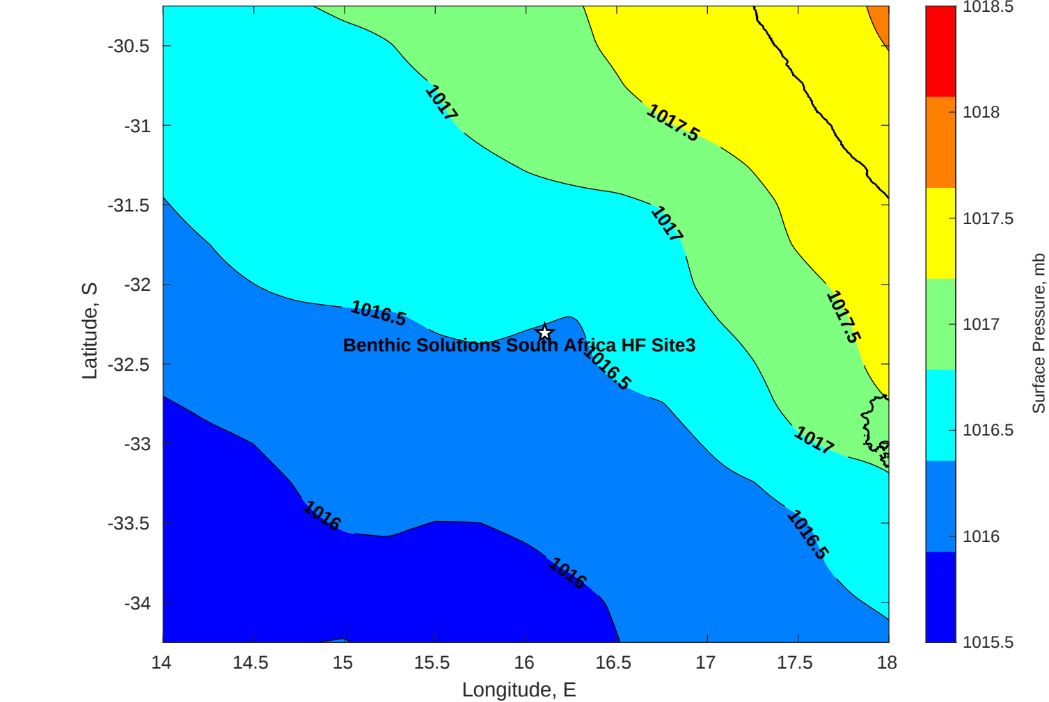
Surface Pressure (mb) for Benthic Solutions South Africa HF Site3 at 09-Apr-2025 00:00:00
