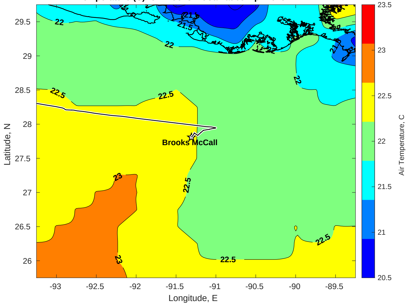
Air Temperature (C) for Brooks McCall at 09-Apr-2025
