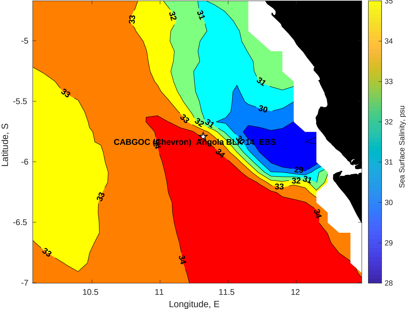
Surface Salinity for CABGOC (Chevron) Angola BLK 14 EBS at 08-Apr-2025 00:00:00
