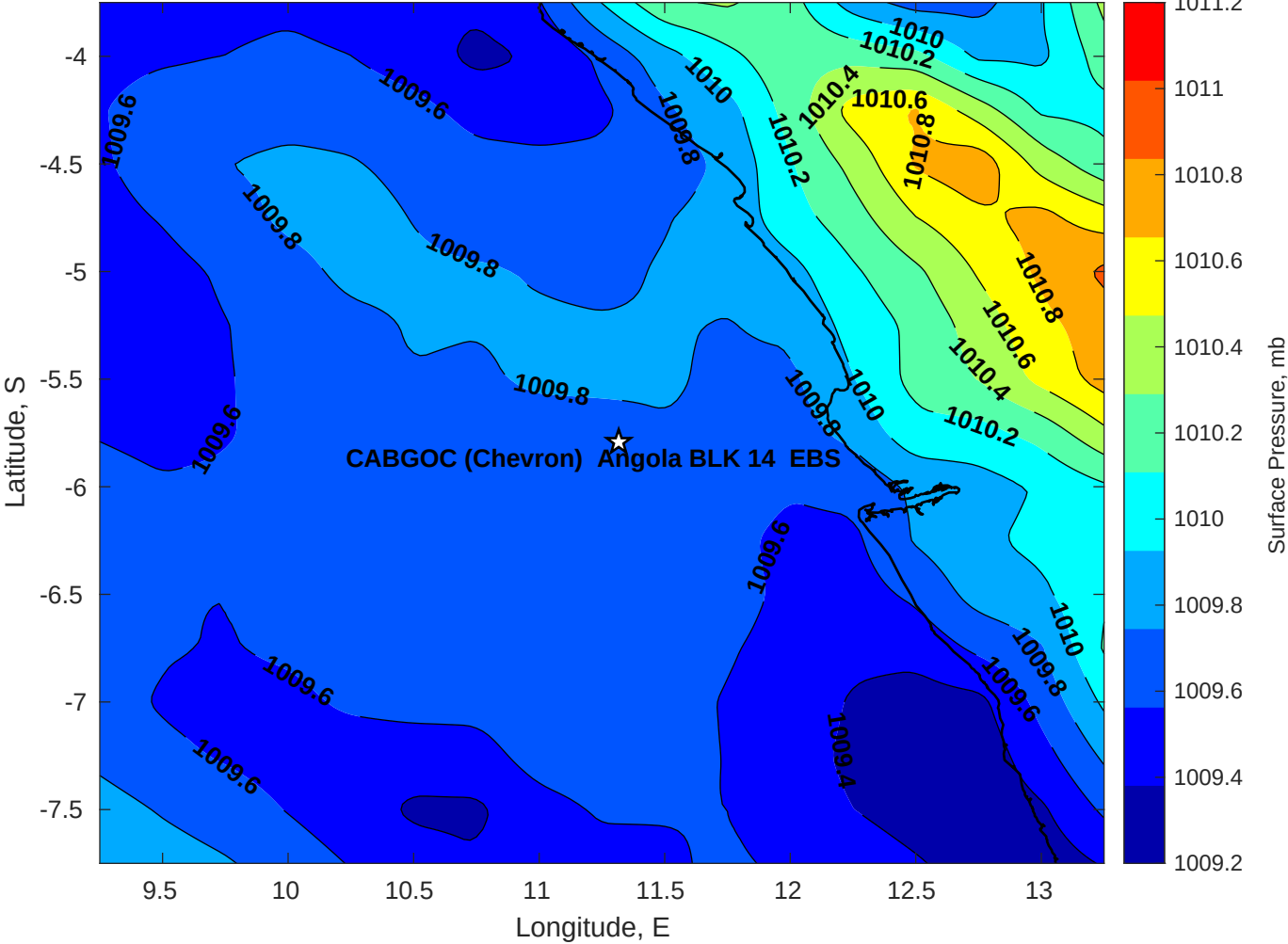
Surface Pressure (mb) for CABGOC (Chevron) Angola BLK 14 EBS at 11-Apr-2025 00:00:00
