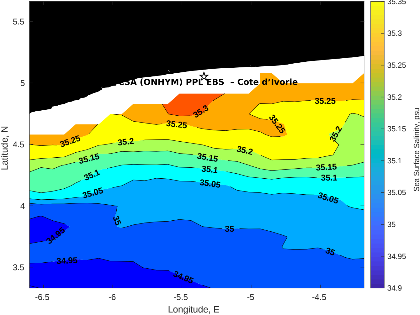
Surface Salinity for CSA (ONHYM) PPL EBS - Cote d'Ivoire at 08-Apr-2025 00:00:00
