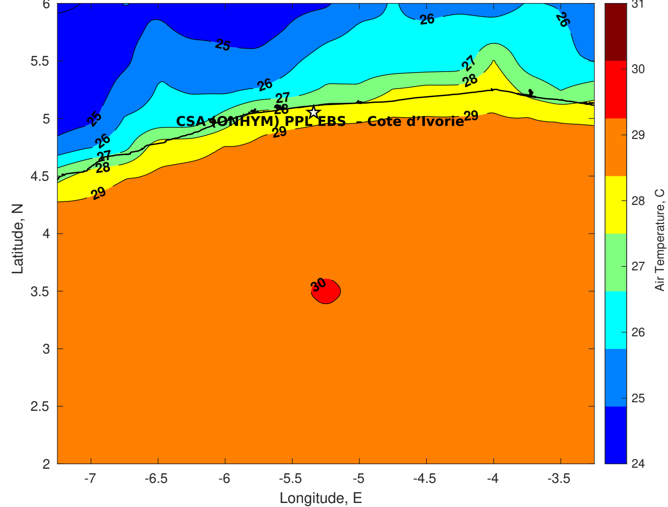
Air Temperature (C) for CSA (ONHYM) PPL EBS - Cote d'Ivoire at 09-Apr-2025
