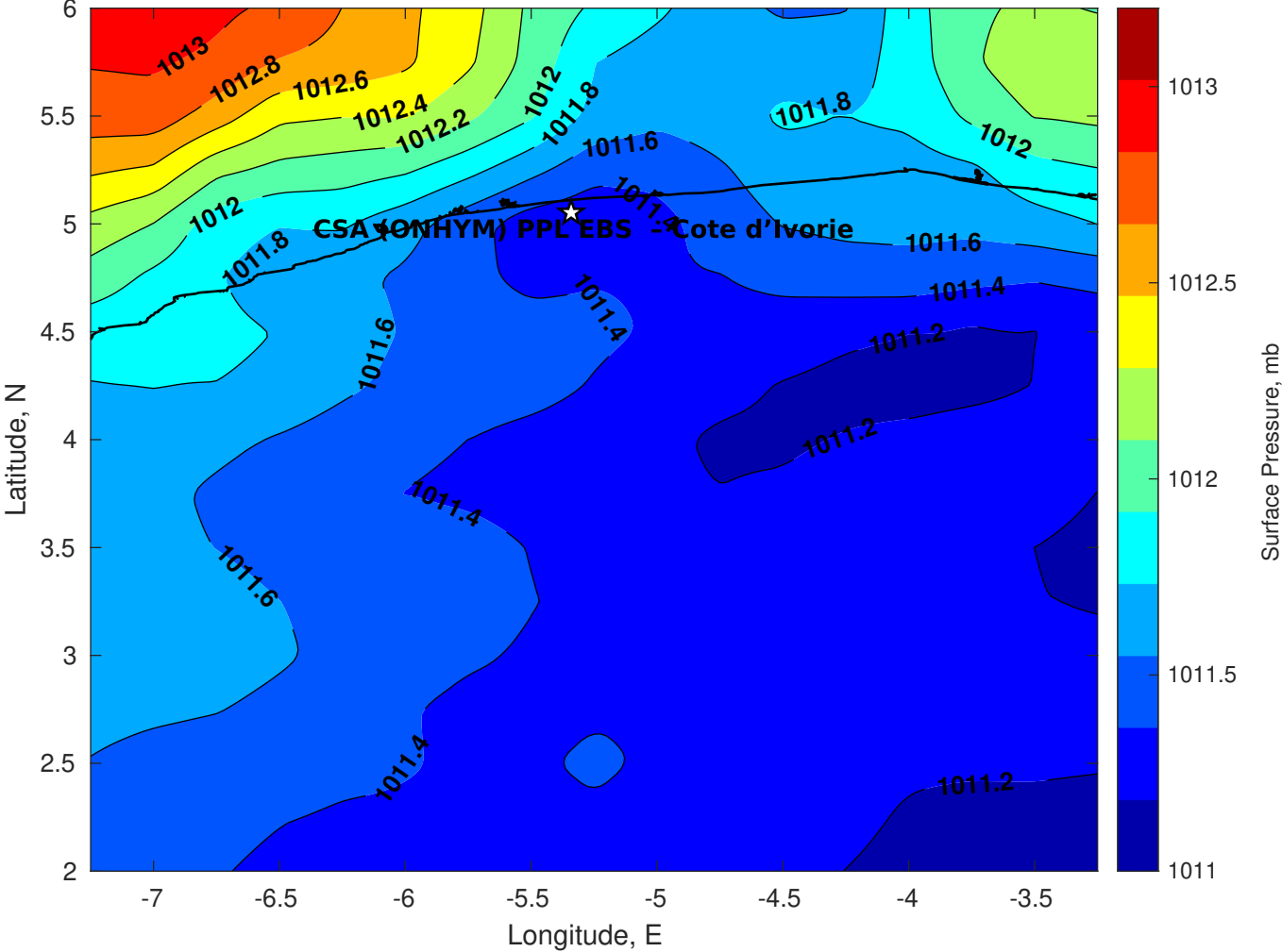
Surface Pressure (mb) for CSA (ONHYM) PPL EBS - Cote d'Ivoire at 10-Apr-2025 00:00:00
