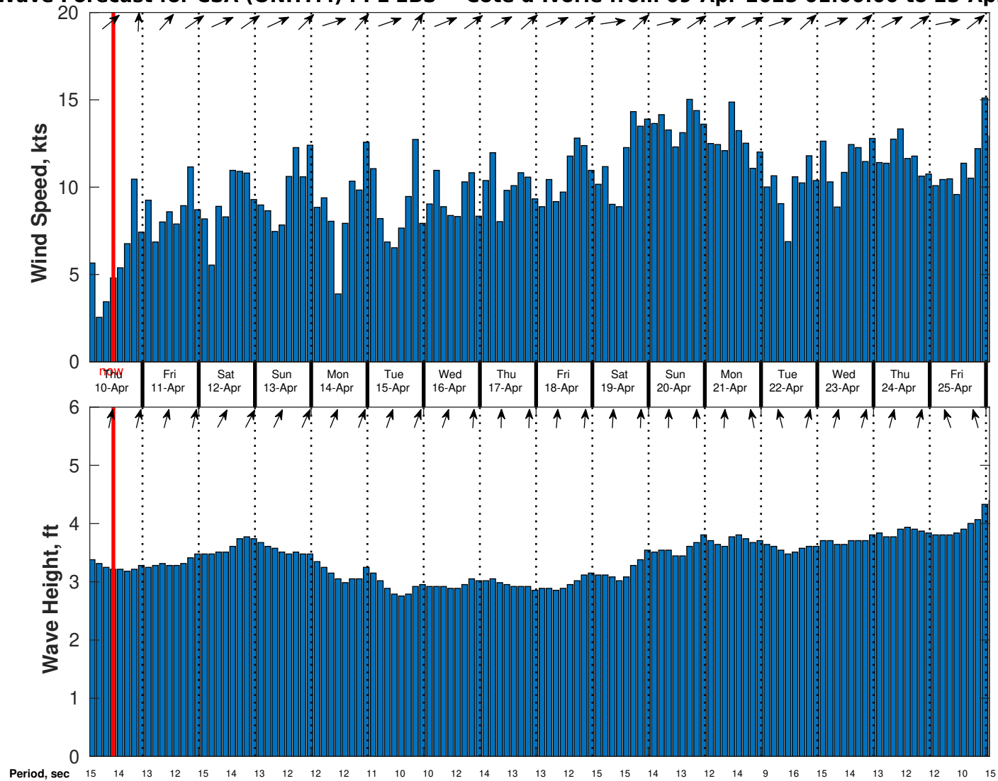
Wind & Wave Forecast for CSA (ONHYM) PPL EBS - Cote d'Ivoire from 09-Apr-2025 01:00:00 to 25-Apr-2025 01:00:00
