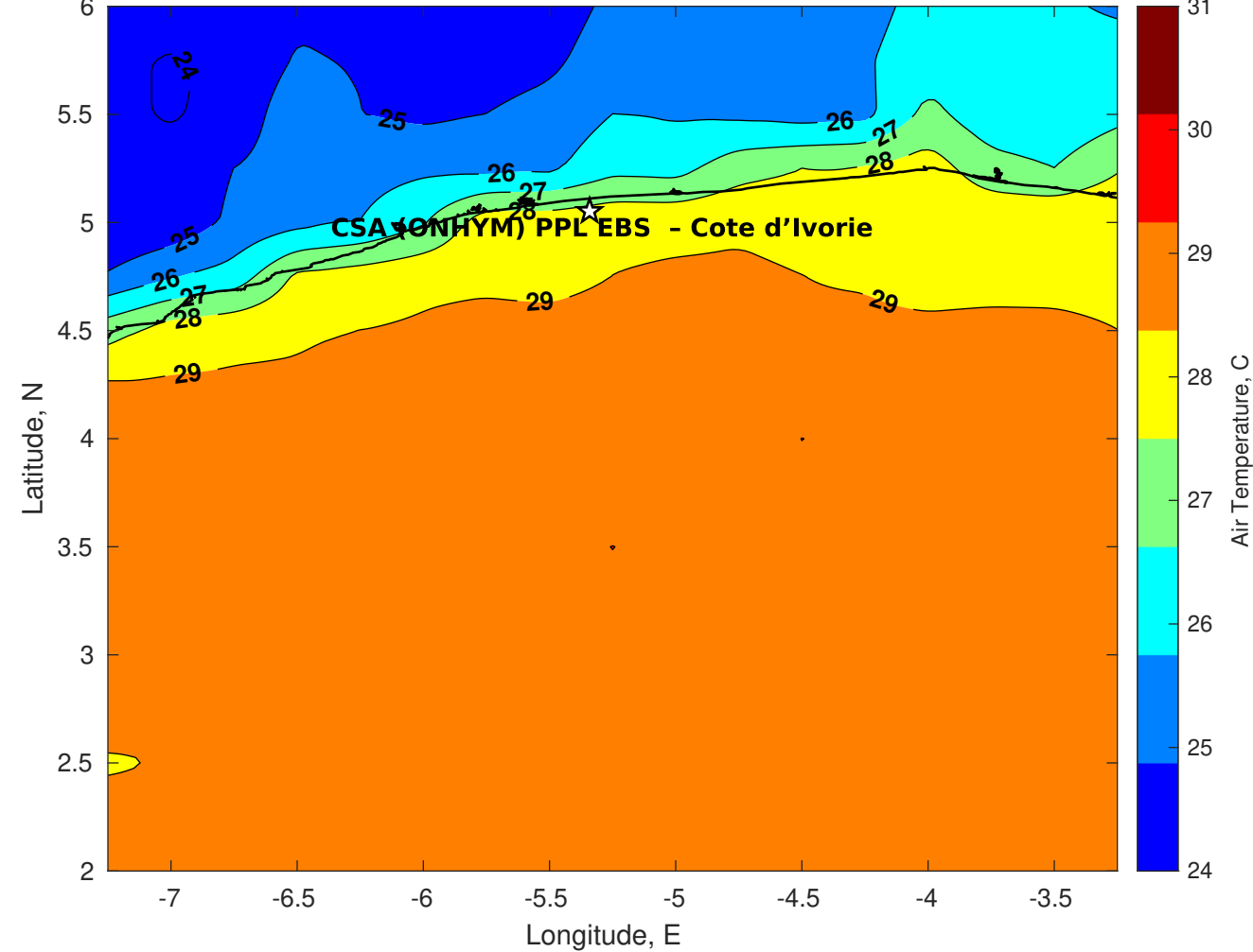
Air Temperature (C) for CSA (ONHYM) PPL EBS - Cote d'Ivoire at 09-Apr-2025
