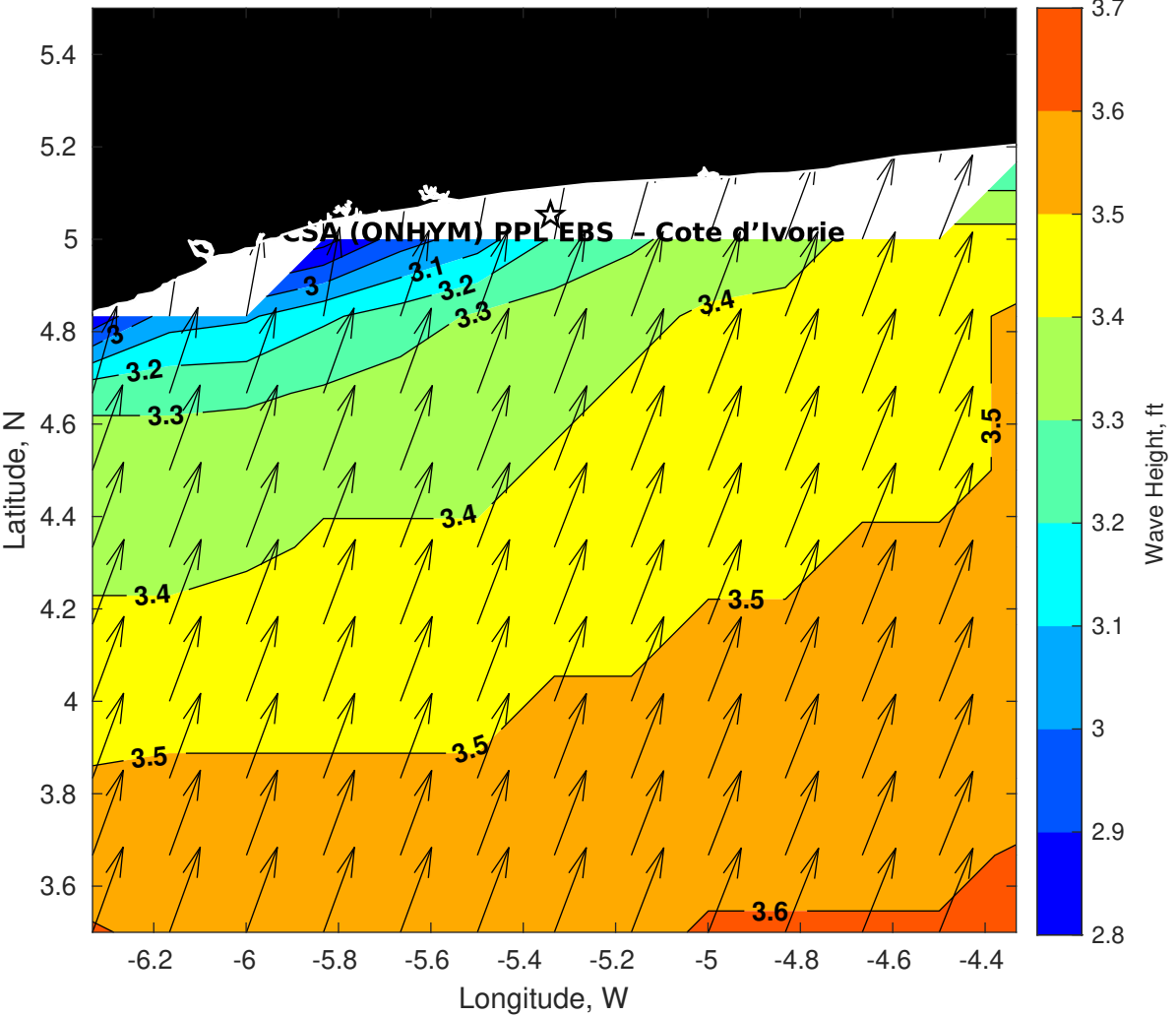
Wave Height (ft) for CSA (ONHYM) PPL EBS - Cote d'Ivoire at 09-Apr-2025 09:00:00
