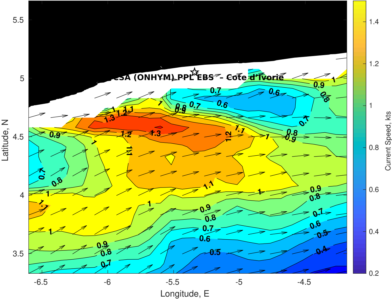
Surface Currents for CSA (ONHYM) PPL EBS - Cote d'Ivoire at 08-Apr-2025 00:00:00
