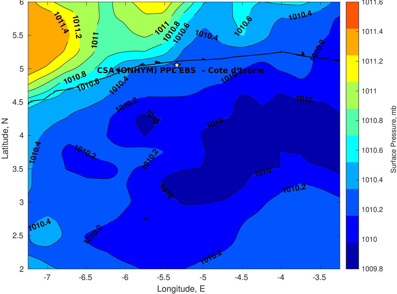
Surface Pressure (mb) for CSA (ONHYM) PPL EBS - Cote d'Ivoire at 11-Apr-2025 00:00:00
