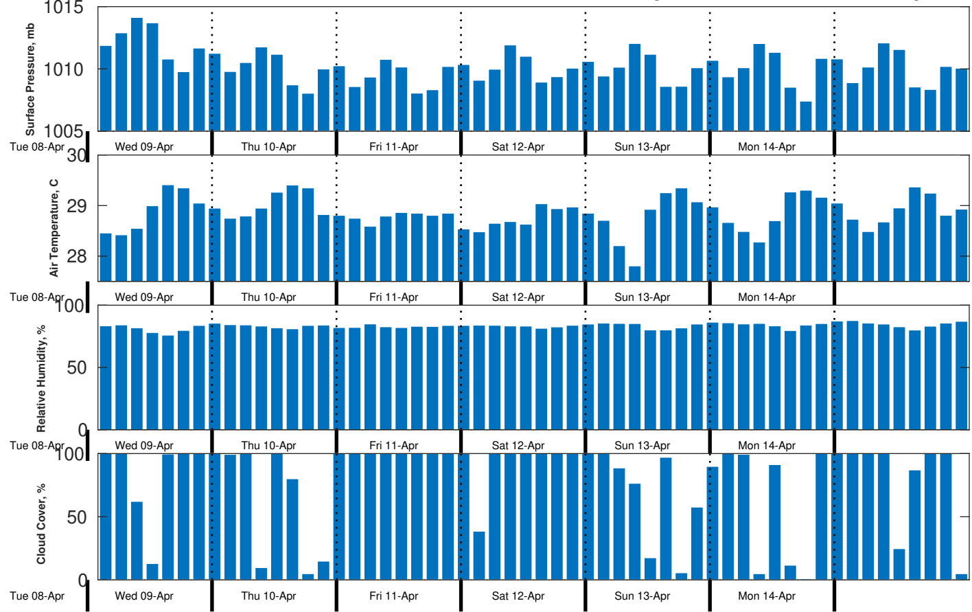
Met Forecast for CSA (ONHYM) PPL EBS - Cote d'Ivoire from 09-Apr-2025 00:00:00 to 16-Apr-2025 00:00:00
