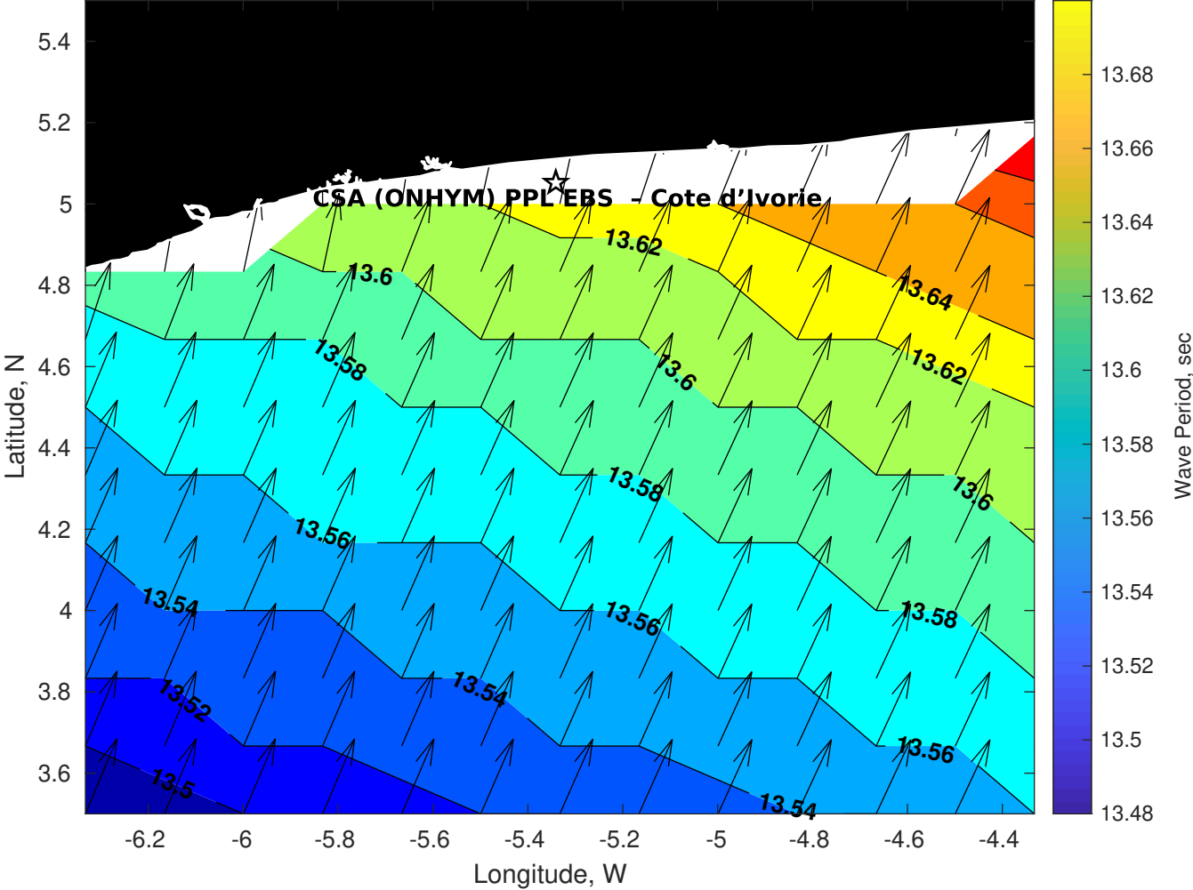
Wave Period (sec) for CSA (ONHYM) PPL EBS - Cote d'Ivoire at 09-Apr-2025 09:00:00
