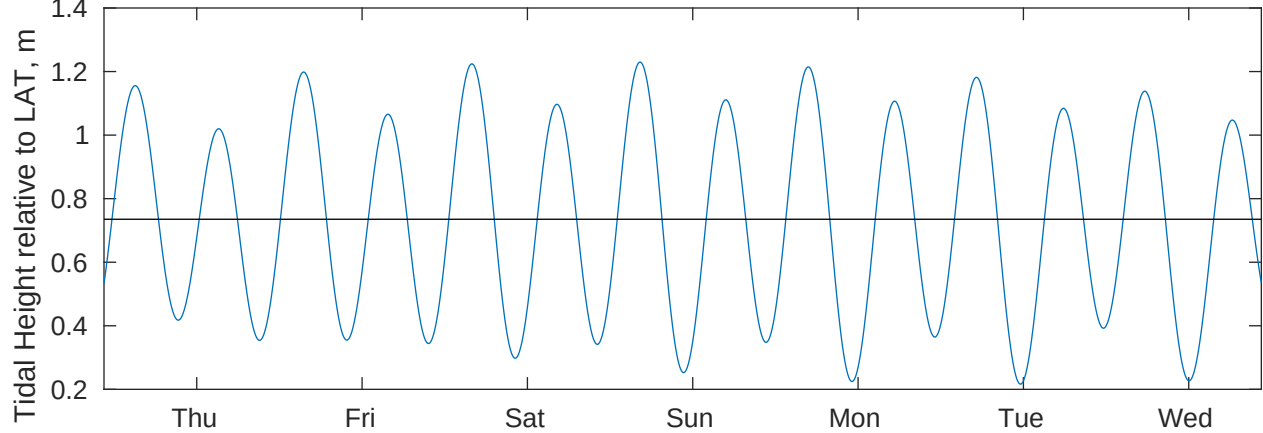
Tidal Currents and Heights for CSA (ONHYM) PPL EBS - Cote d'Ivoire at 20250409
