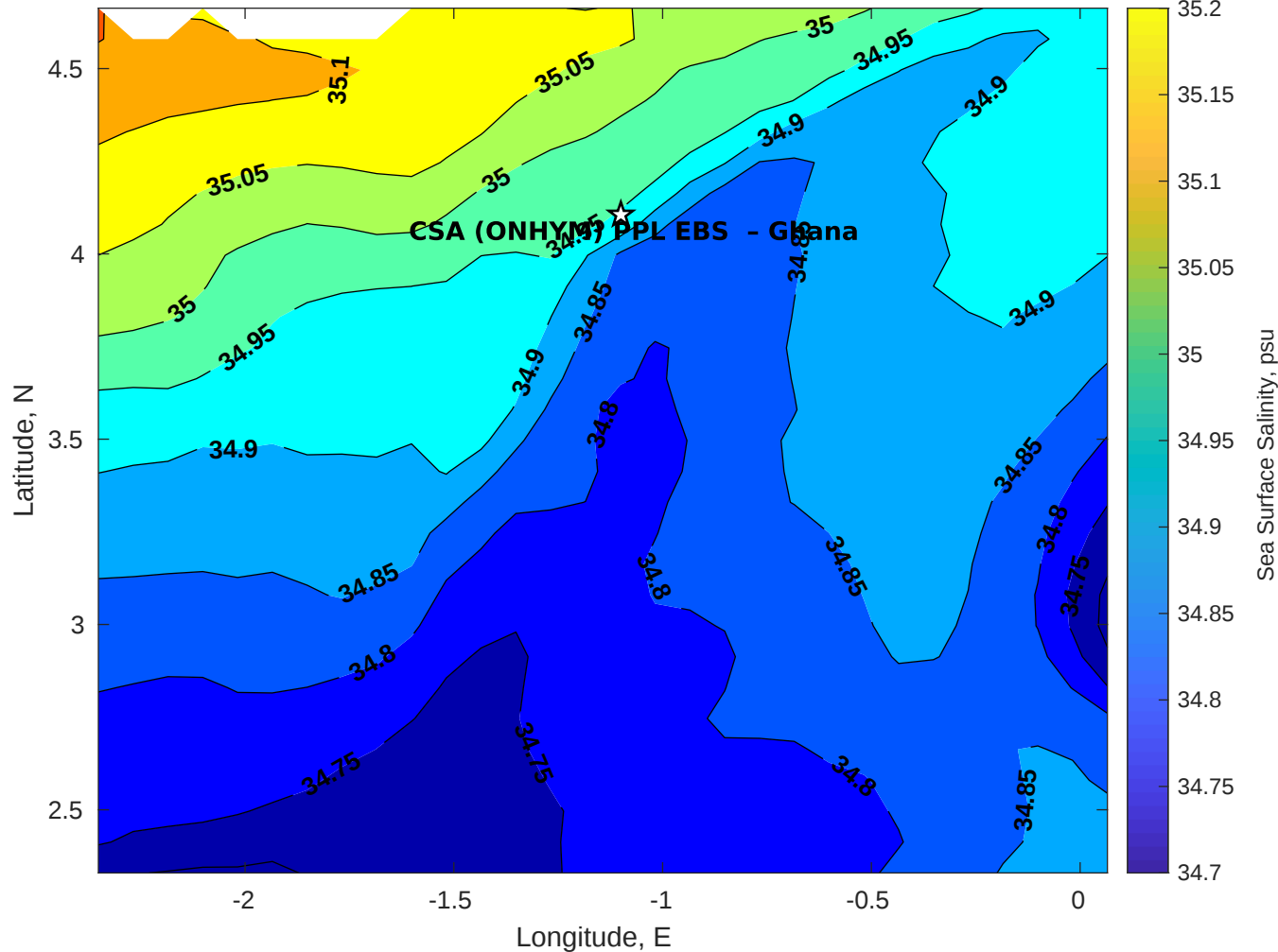
Surface Salinity for CSA (ONHYM) PPL EBS - Ghana at 08-Apr-2025 00:00:00
