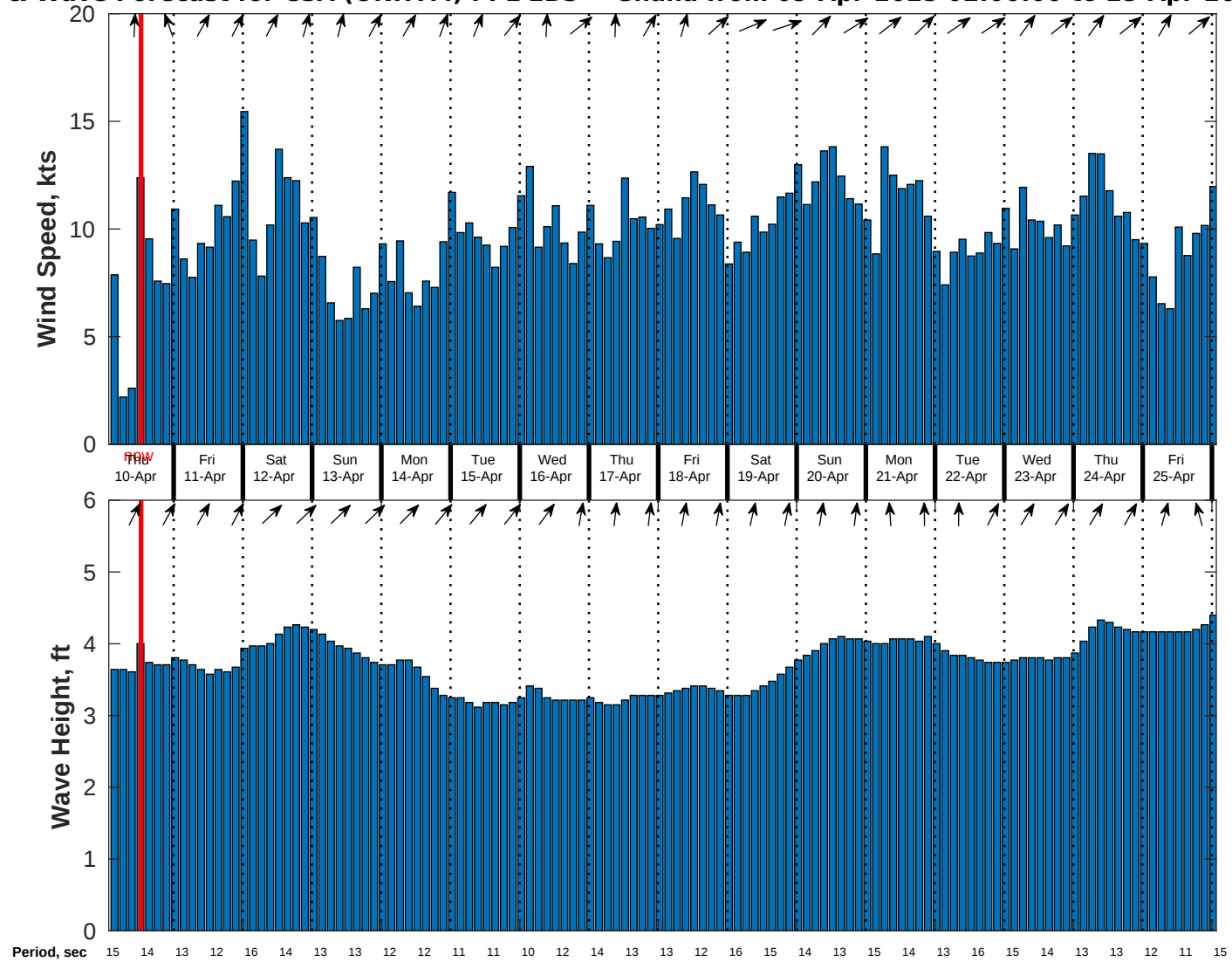
Wind & Wave Forecast for CSA (ONHYM) PPL EBS - Ghana from 09-Apr-2025 02:00:00 to 25-Apr-2025 02:00:00
