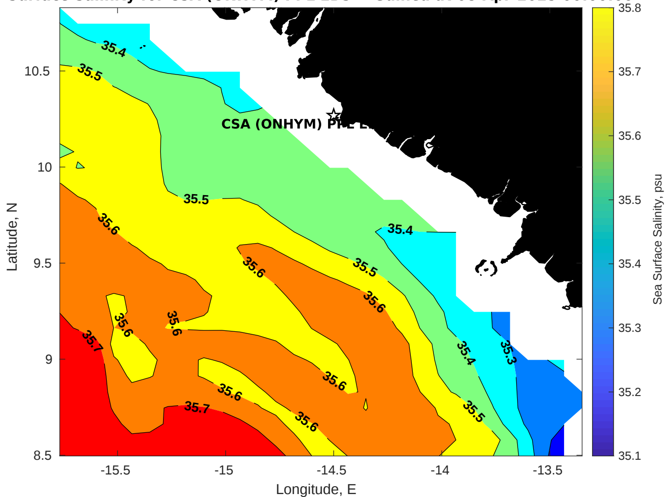
Surface Salinity for CSA (ONHYM) PPL EBS - Guinea at 08-Apr-2025 00:00:00
