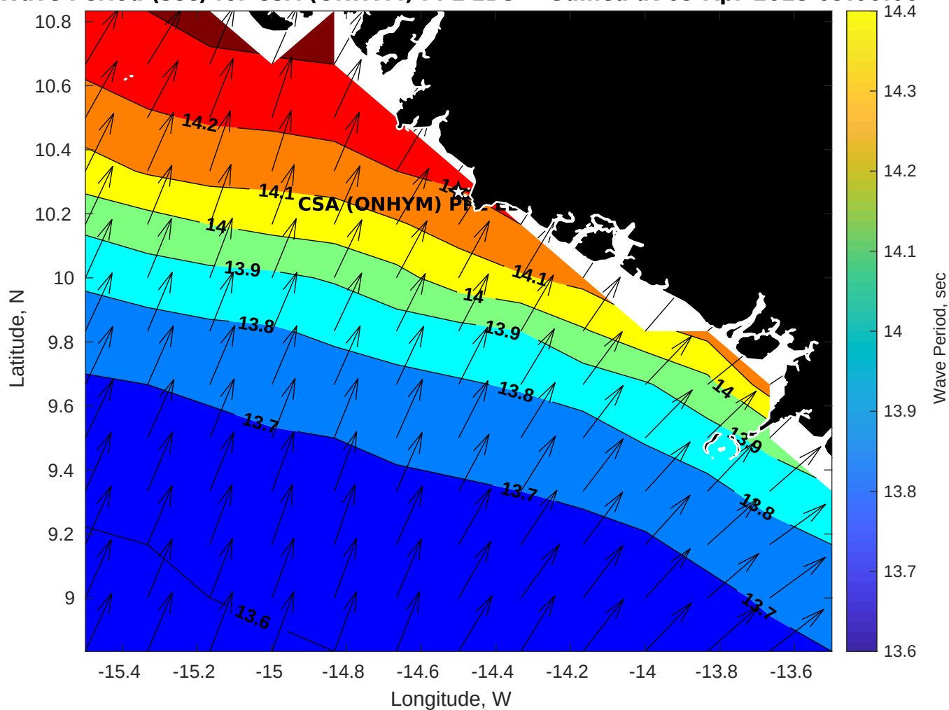
Wave Period (sec) for CSA (ONHYM) PPL EBS - Guinea at 09-Apr-2025 09:00:00
