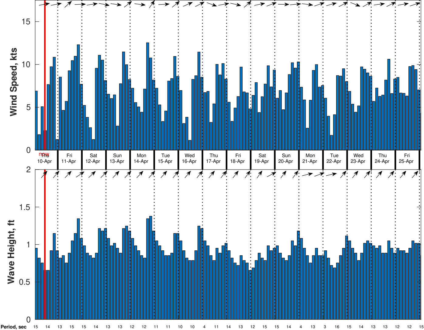
Wind & Wave Forecast for CSA (ONHYM) PPL EBS - Guinea from 09-Apr-2025 01:00:00 to 25-Apr-2025 01:00:00
