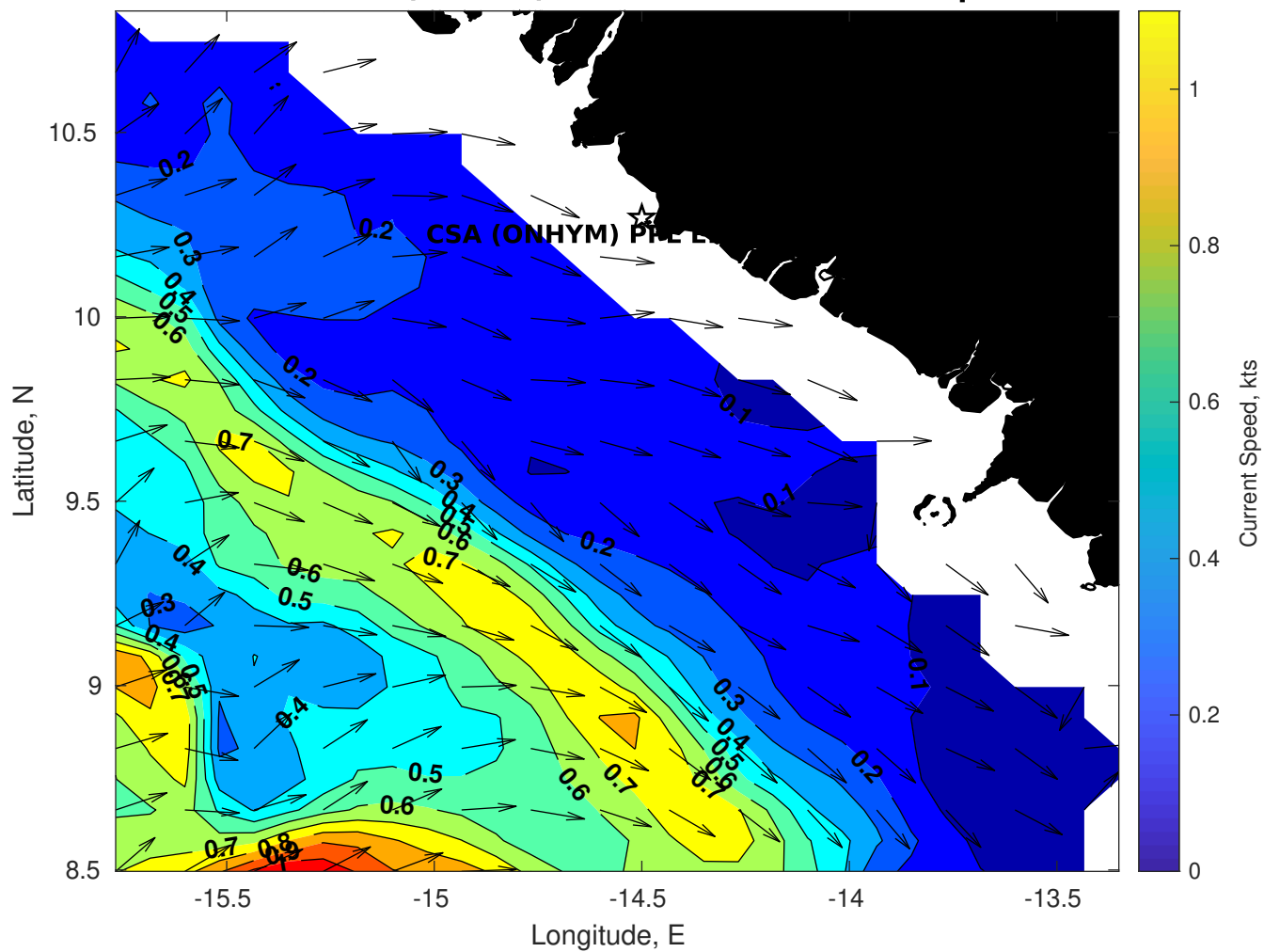
Surface Currents for CSA (ONHYM) PPL EBS - Guinea at 08-Apr-2025 00:00:00
