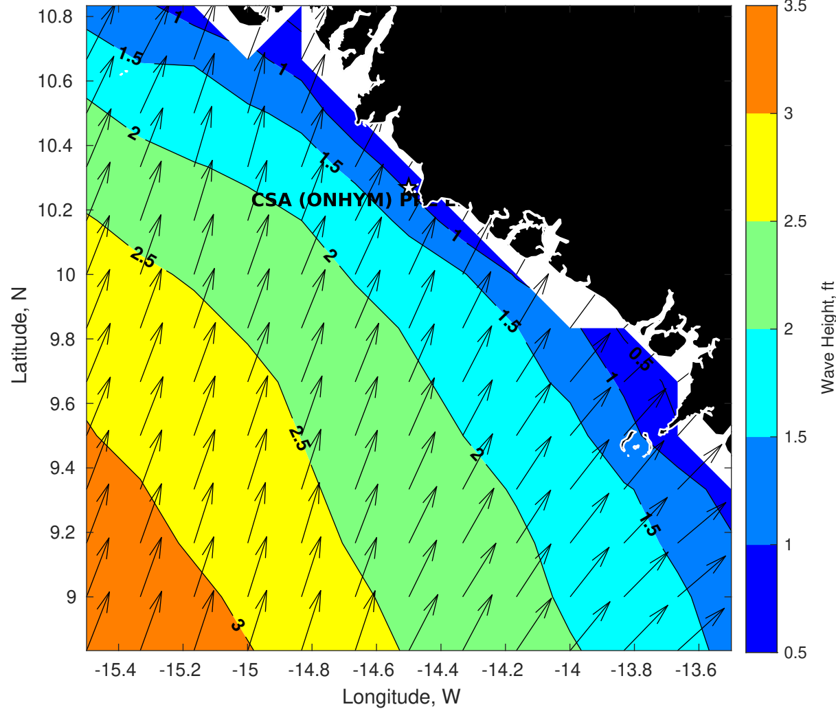
Wave Height (ft) for CSA (ONHYM) PPL EBS - Guinea at 09-Apr-2025 09:00:00
