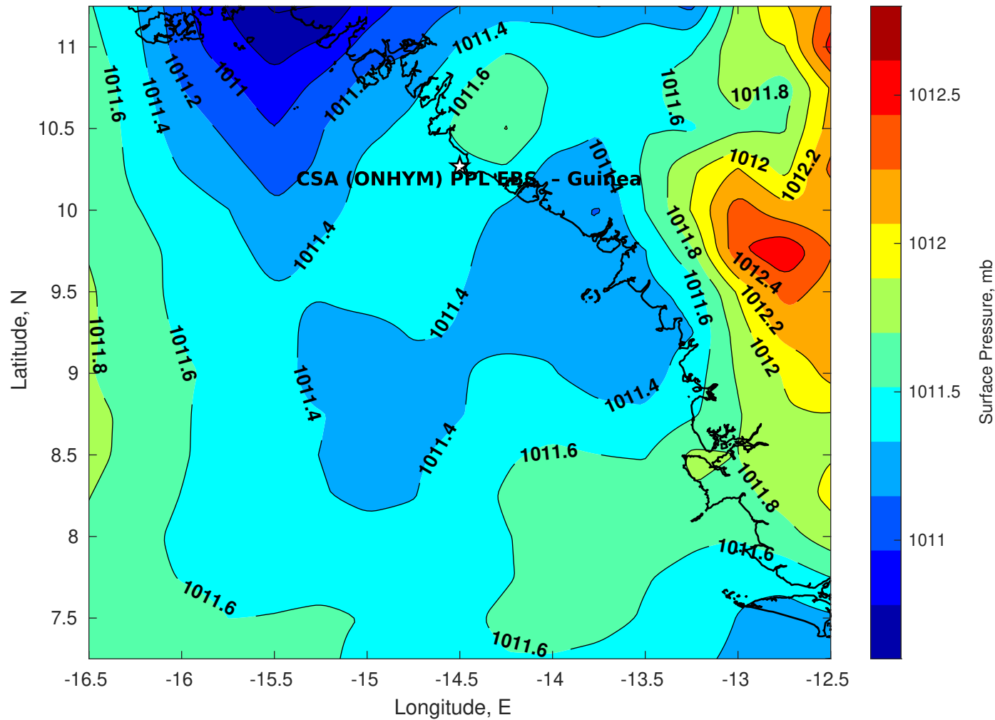
Surface Pressure (mb) for CSA (ONHYM) PPL EBS - Guinea at 11-Apr-2025 00:00:00
