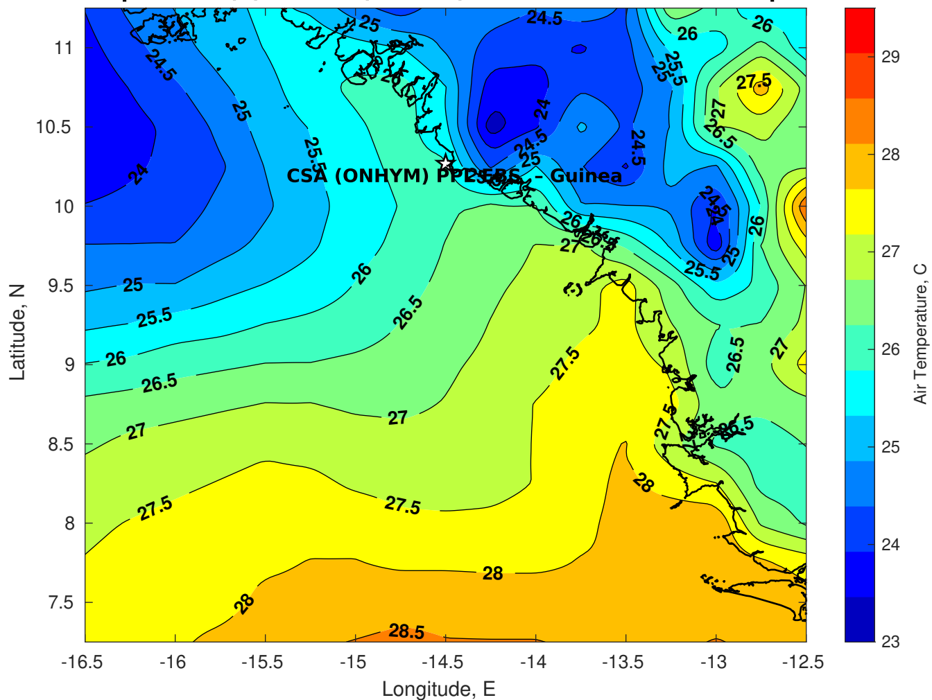
Air Temperature (C) for CSA (ONHYM) PPL EBS - Guinea at 09-Apr-2025
