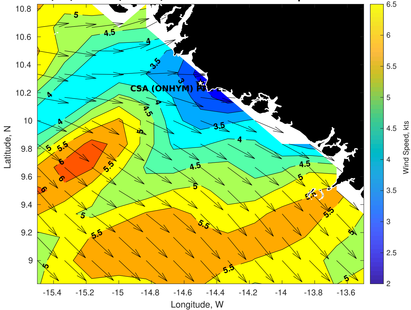
Winds (kts) for CSA (ONHYM) PPL EBS - Guinea at 09-Apr-2025 09:00:00
