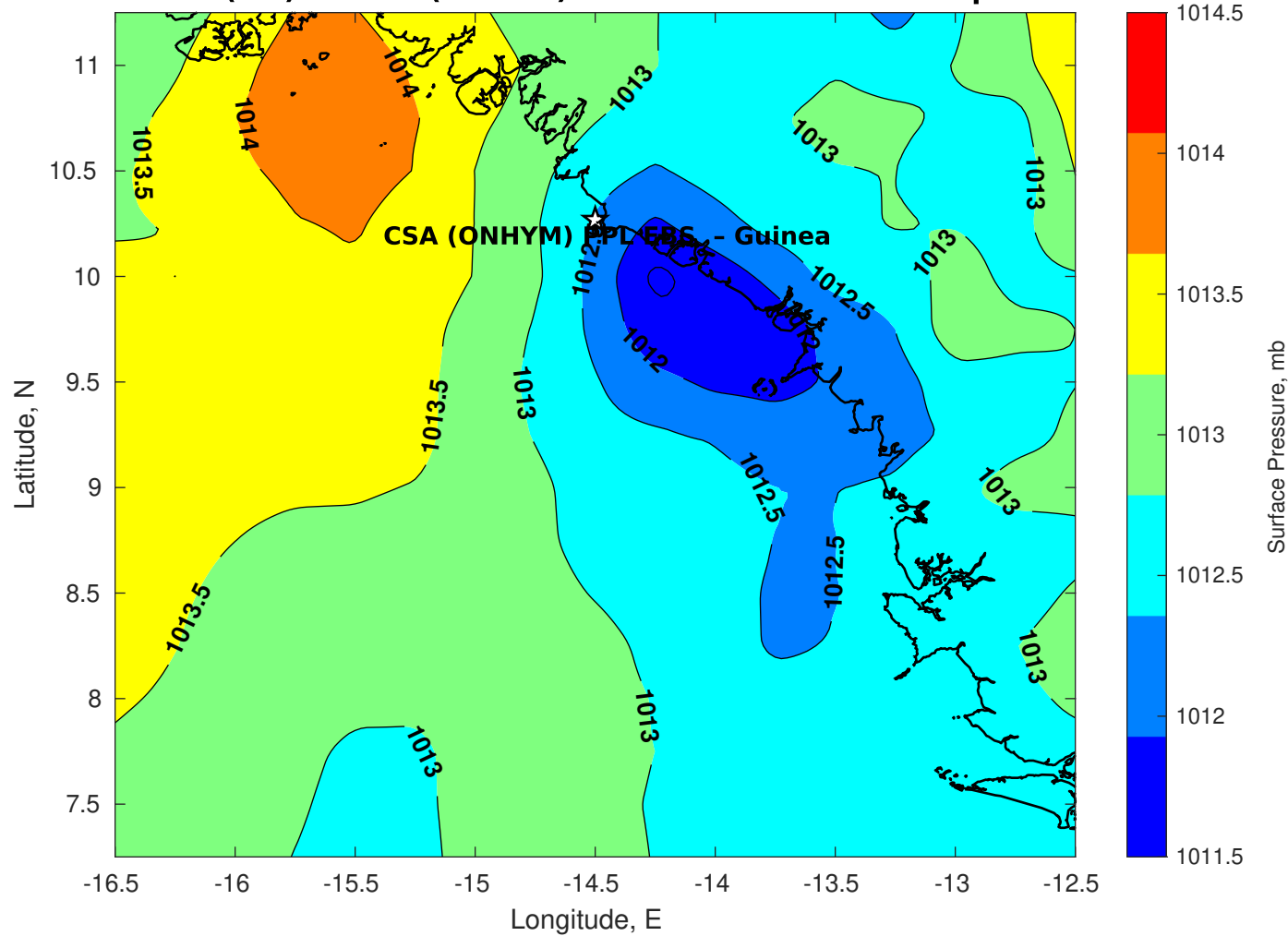
Surface Pressure (mb) for CSA (ONHYM) PPL EBS - Guinea at 10-Apr-2025 00:00:00
