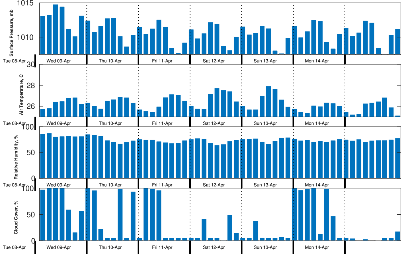
Met Forecast for CSA (ONHYM) PPL EBS - Guinea from 09-Apr-2025 00:00:00 to 16-Apr-2025 00:00:00
