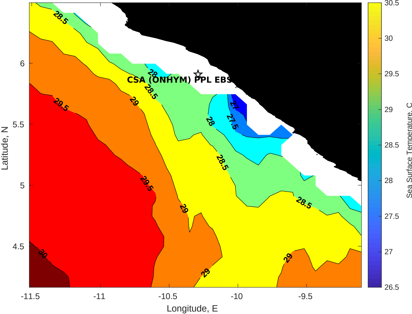
SST for CSA (ONHYM) PPL EBS - Liberia at 08-Apr-2025 00:00:00
