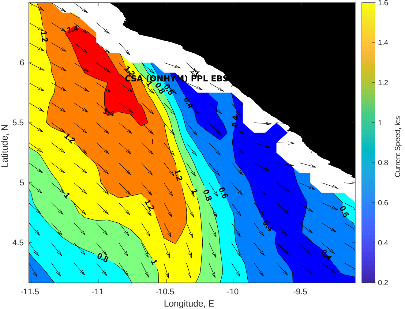
Surface Currents for CSA (ONHYM) PPL EBS - Liberia at 08-Apr-2025 00:00:00
