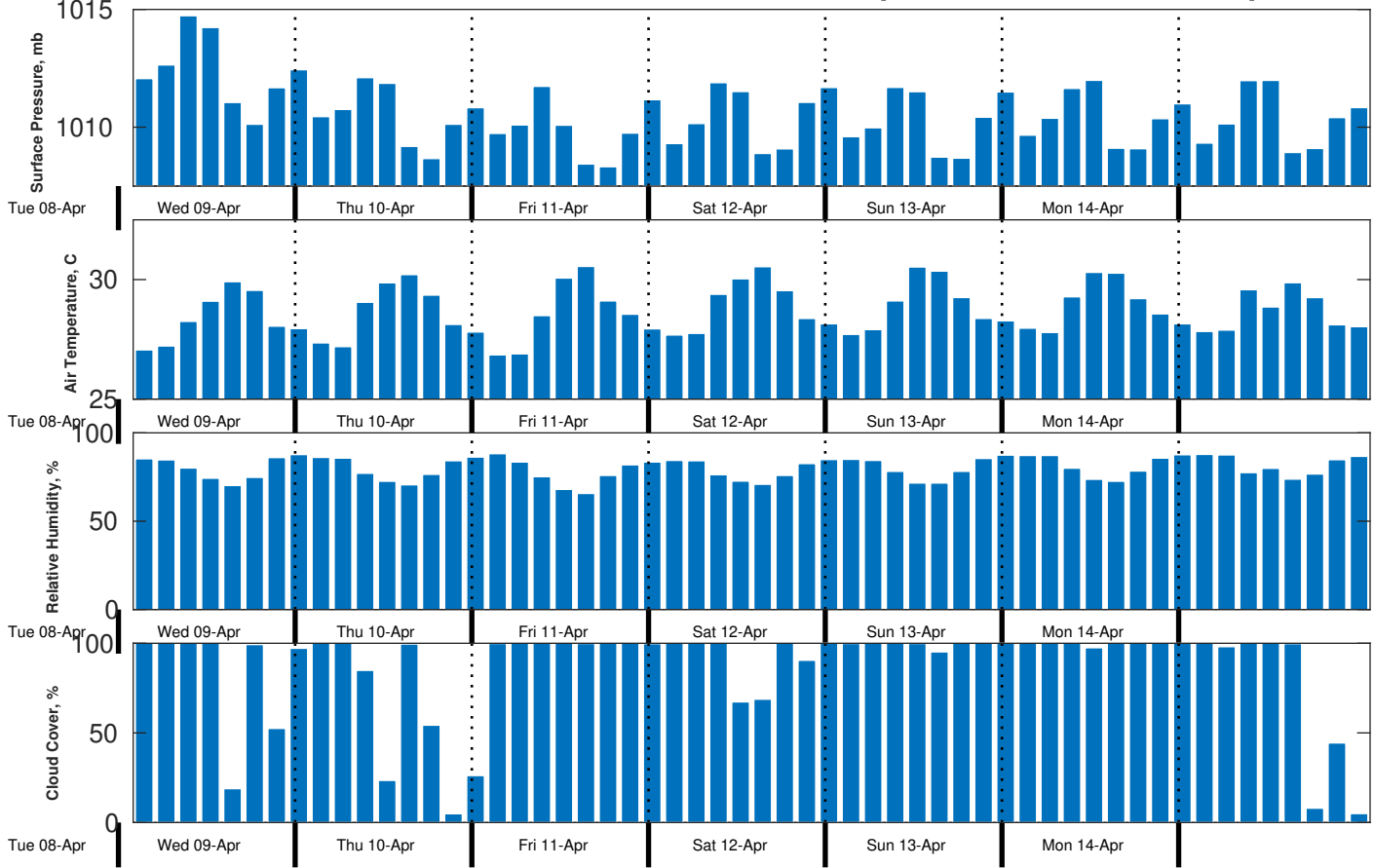
Met Forecast for CSA (ONHYM) PPL EBS - Liberia from 09-Apr-2025 00:00:00 to 16-Apr-2025 00:00:00
