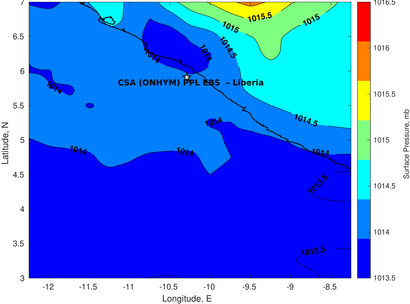
Surface Pressure (mb) for CSA (ONHYM) PPL EBS - Liberia at 09-Apr-2025 00:00:00
