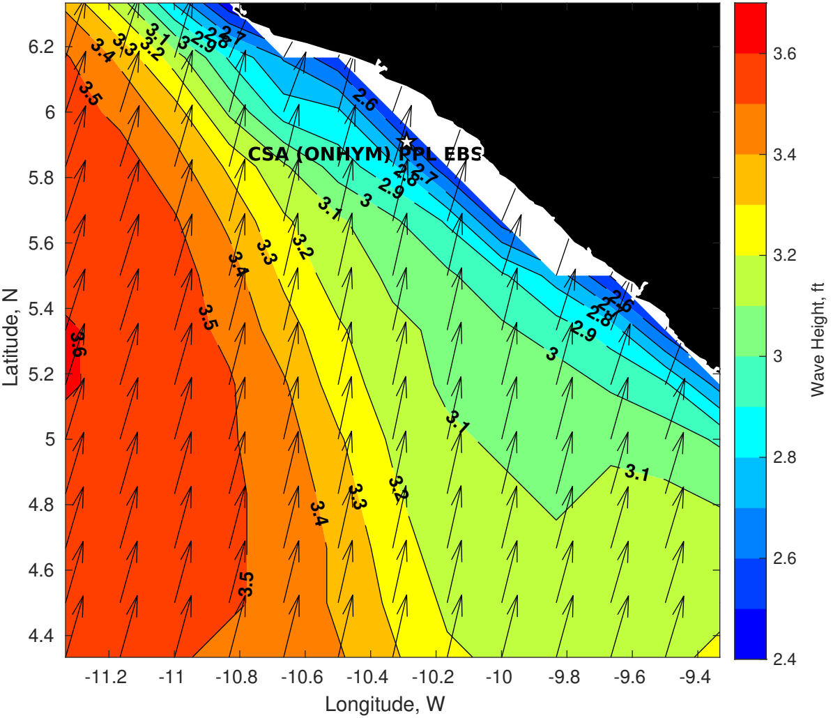
Wave Height (ft) for CSA (ONHYM) PPL EBS - Liberia at 09-Apr-2025 09:00:00
