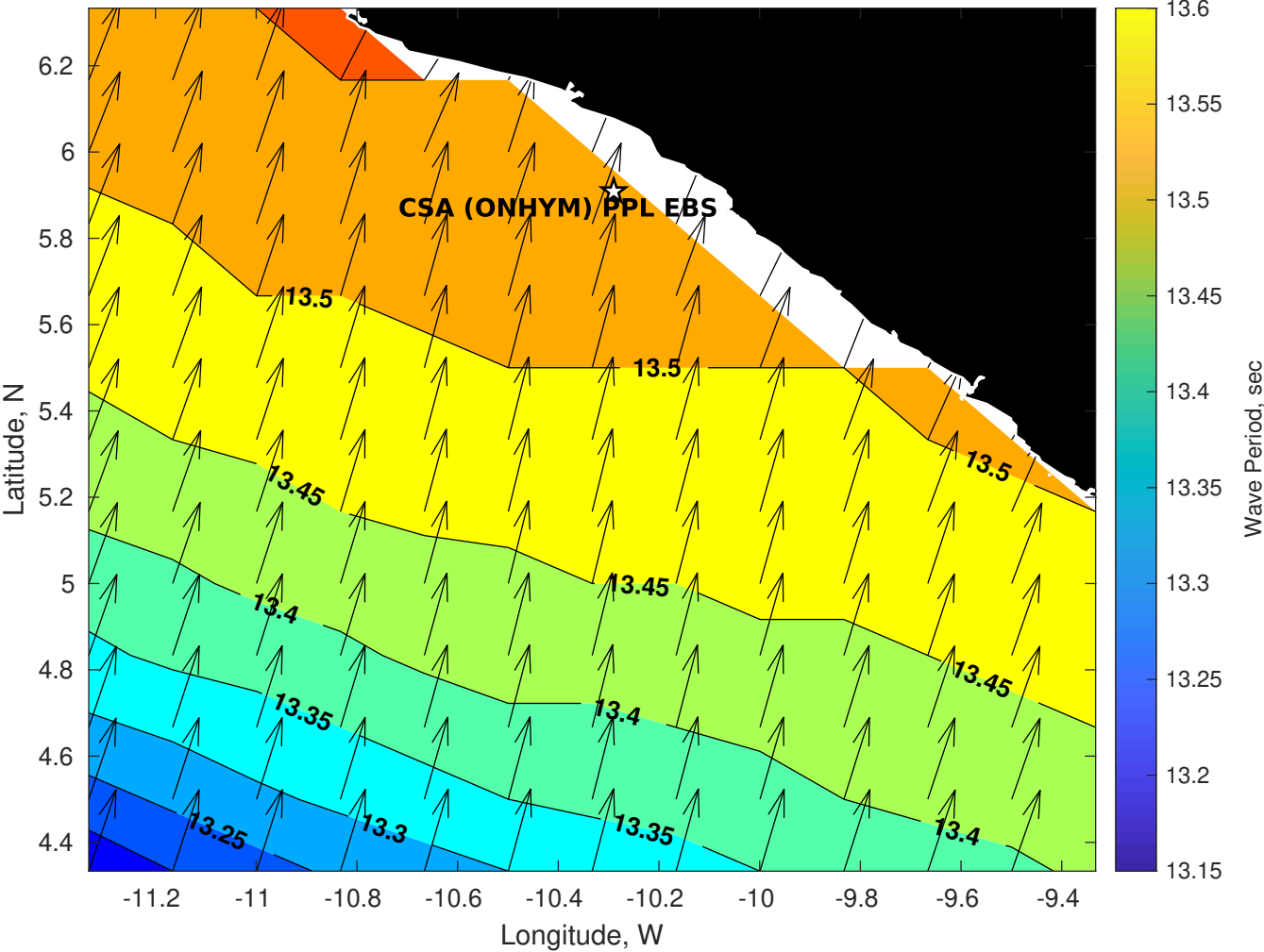
Wave Period (sec) for CSA (ONHYM) PPL EBS - Liberia at 09-Apr-2025 09:00:00
