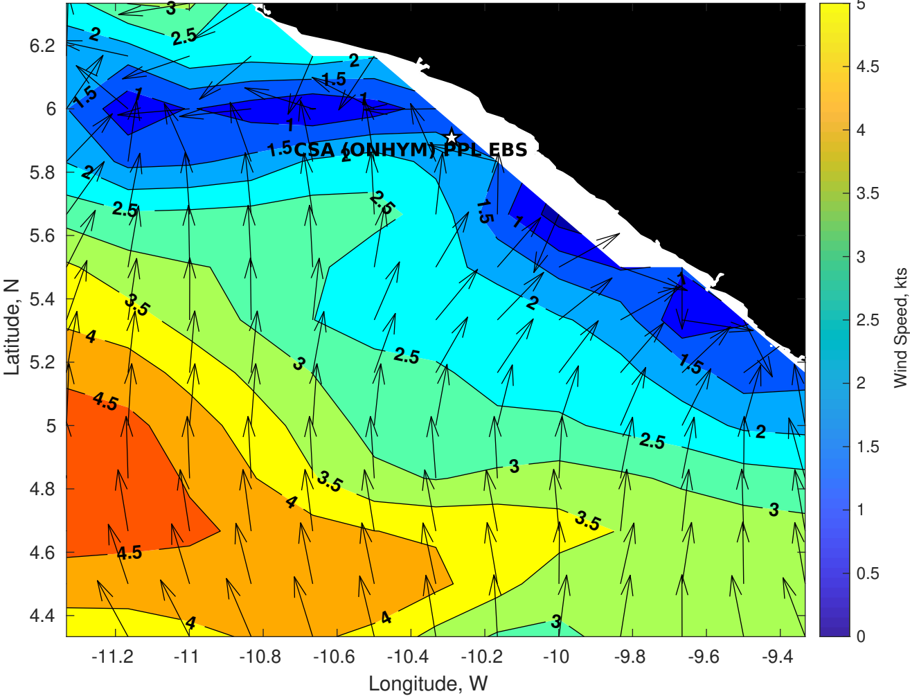
Winds (kts) for CSA (ONHYM) PPL EBS - Liberia at 09-Apr-2025 09:00:00
