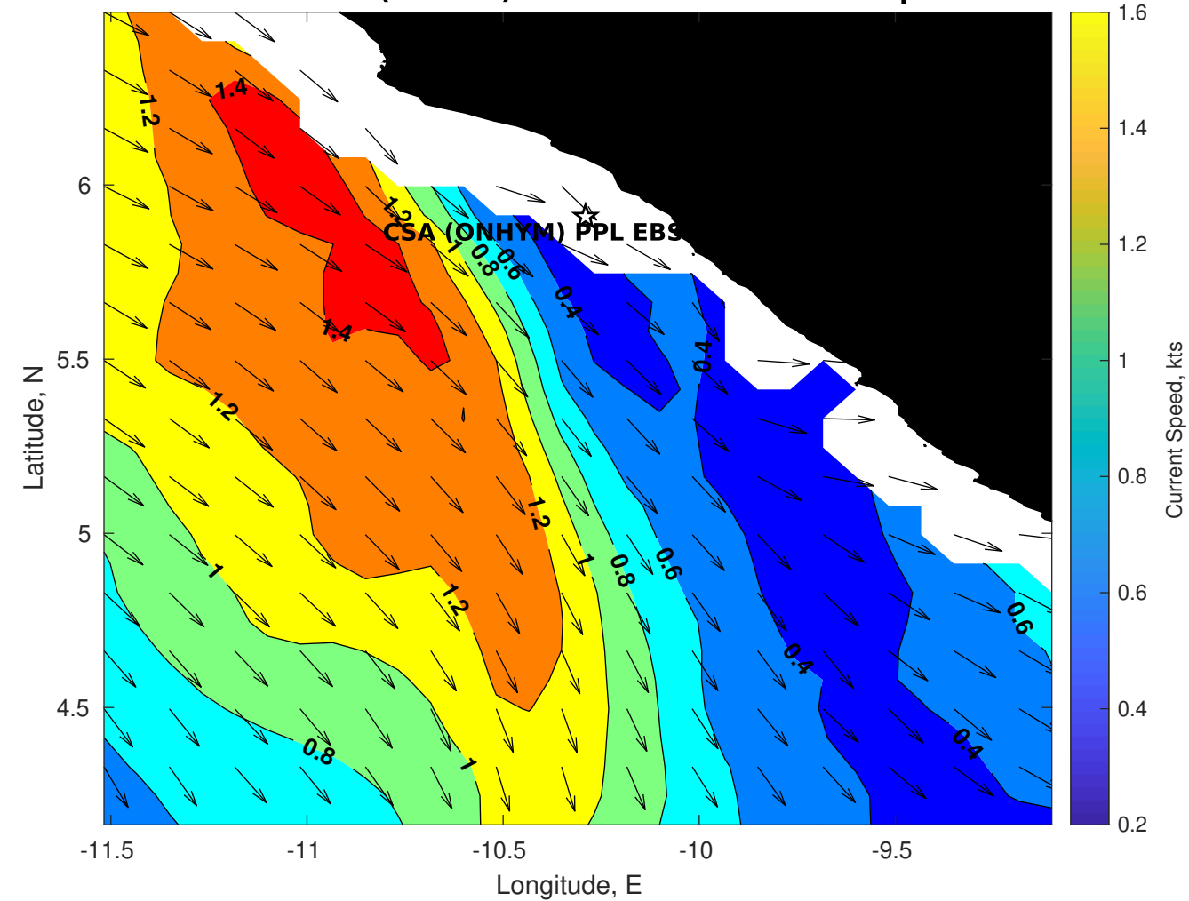
Surface Currents for CSA (ONHYM) PPL EBS - Liberia at 08-Apr-2025 00:00:00
