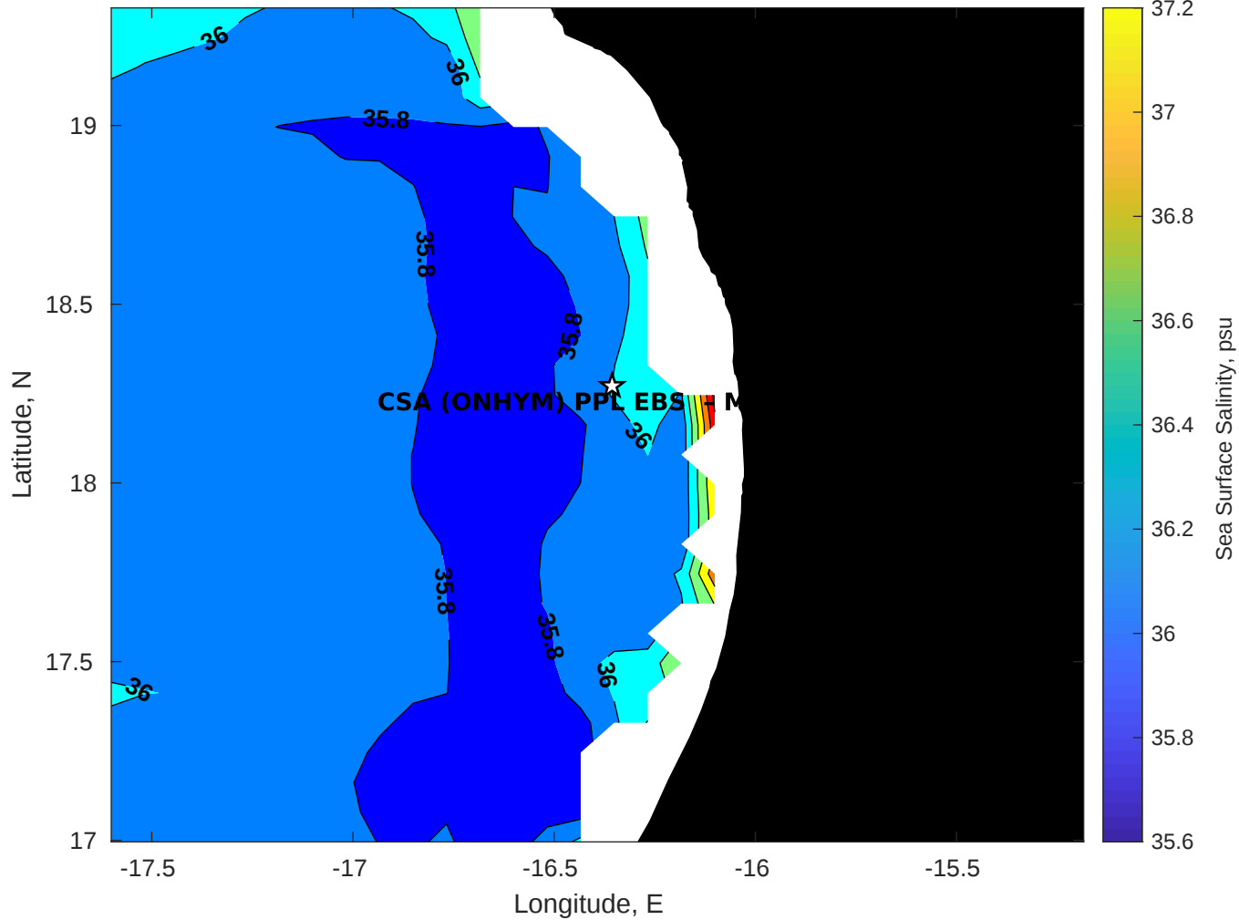
Surface Salinity for CSA (ONHYM) PPL EBS - Mauritania at 08-Apr-2025 00:00:00
