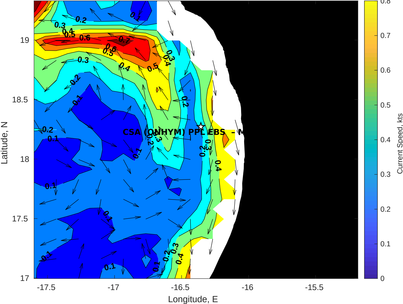
Surface Currents for CSA (ONHYM) PPL EBS - Mauritania at 08-Apr-2025 00:00:00
