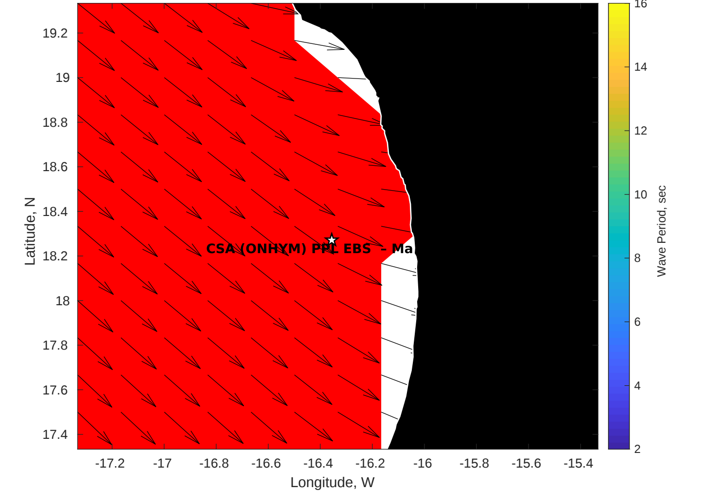
Wave Period (sec) for CSA (ONHYM) PPL EBS - Mauritania at 09-Apr-2025 09:00:00
