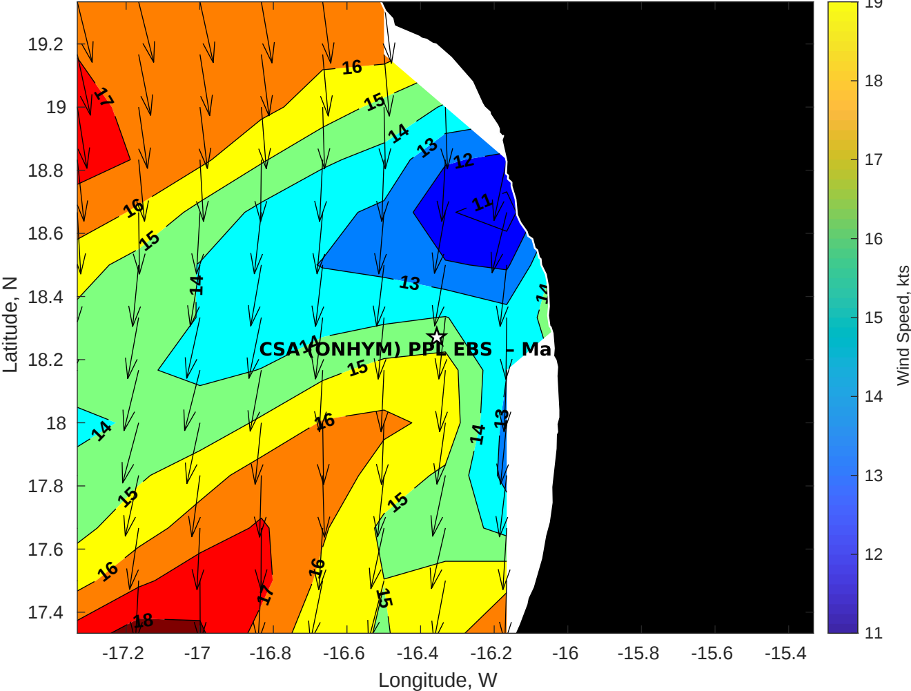
Winds (kts) for CSA (ONHYM) PPL EBS - Mauritania at 09-Apr-2025 09:00:00
