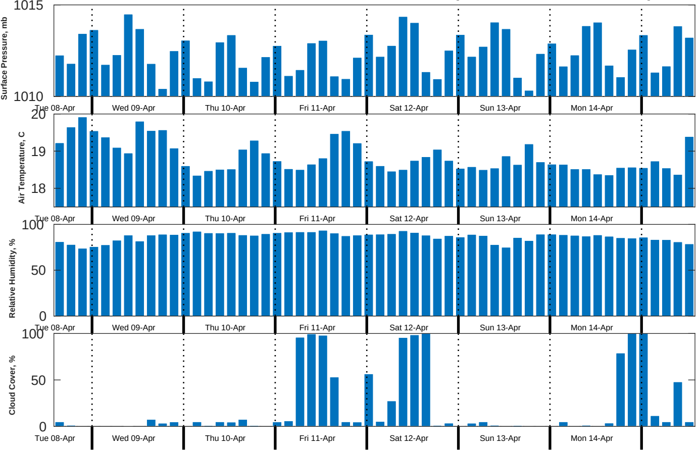
Met Forecast for CSA (ONHYM) PPL EBS - Mauritania from 08-Apr-2025 12:00:00 to 15-Apr-2025 12:00:00
