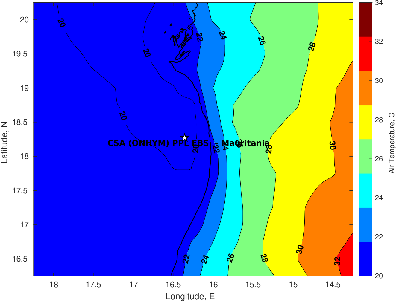
Air Temperature (C) for CSA (ONHYM) PPL EBS - Mauritania at 09-Apr-2025
