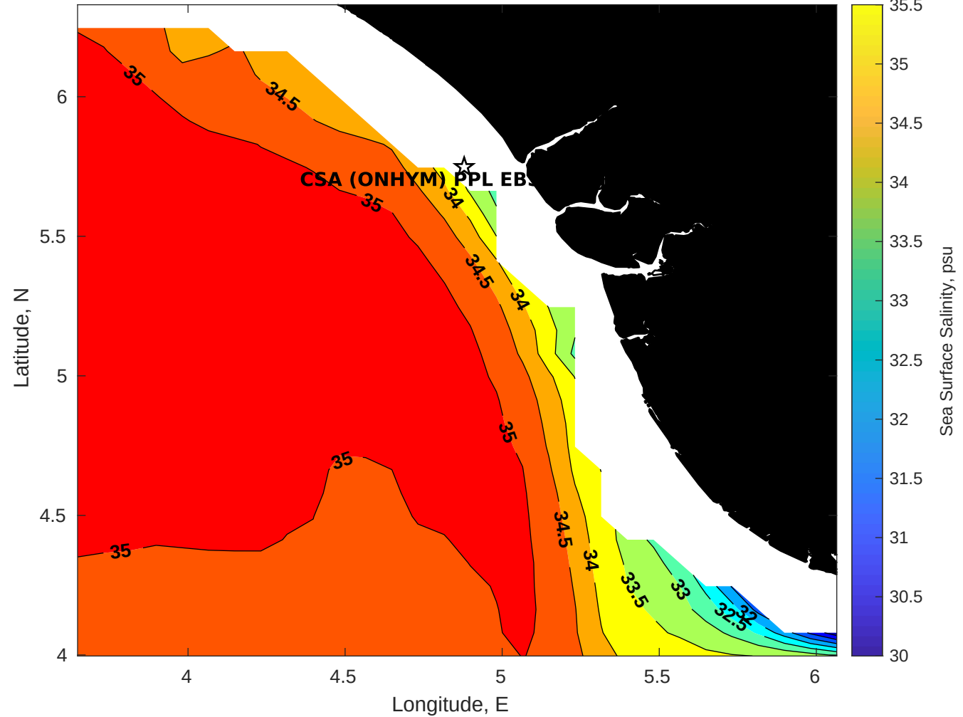
Surface Salinity for CSA (ONHYM) PPL EBS - Nigeria at 08-Apr-2025 00:00:00
