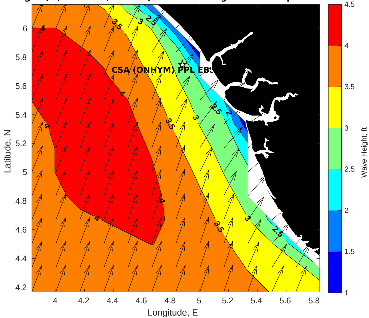
Wave Height (ft) for CSA (ONHYM) PPL EBS - Nigeria at 09-Apr-2025 09:00:00
