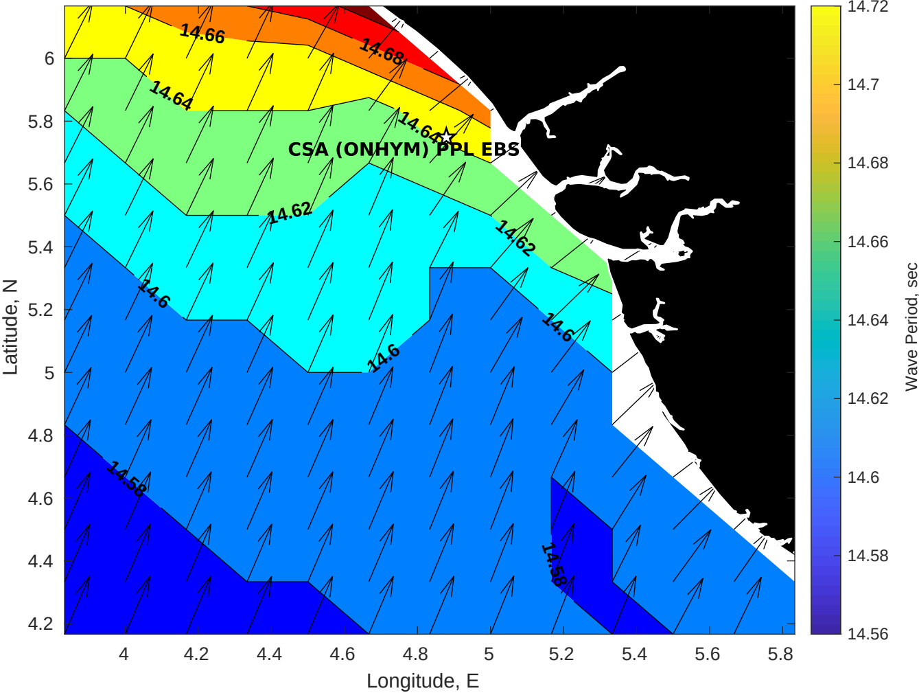
Wave Period (sec) for CSA (ONHYM) PPL EBS - Nigeria at 09-Apr-2025 09:00:00
