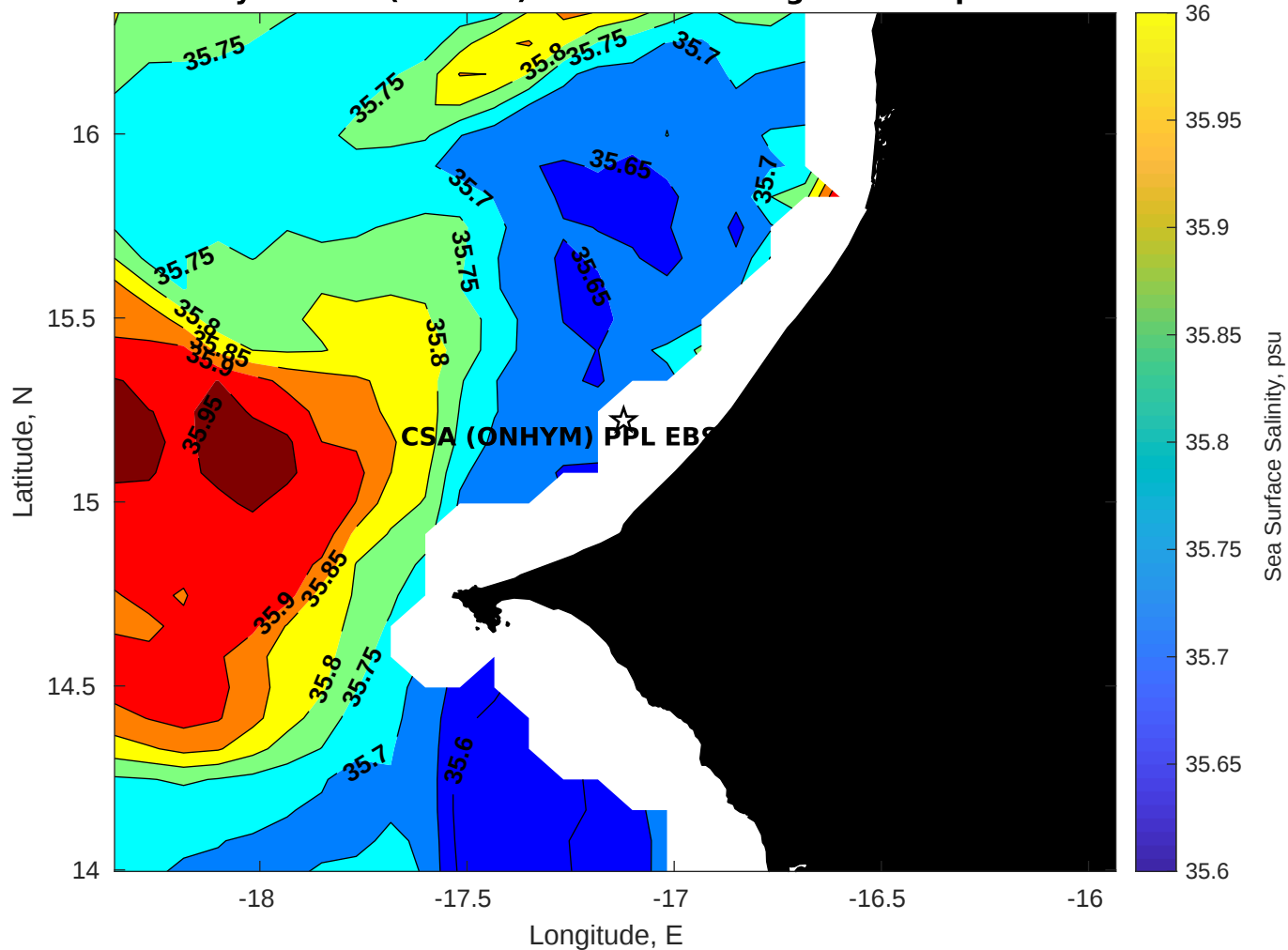
Surface Salinity for CSA (ONHYM) PPL EBS - Senegal at 08-Apr-2025 00:00:00
