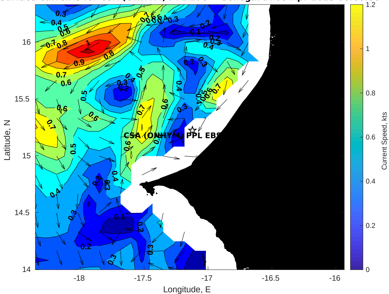
Surface Currents for CSA (ONHYM) PPL EBS - Senegal at 08-Apr-2025 00:00:00
