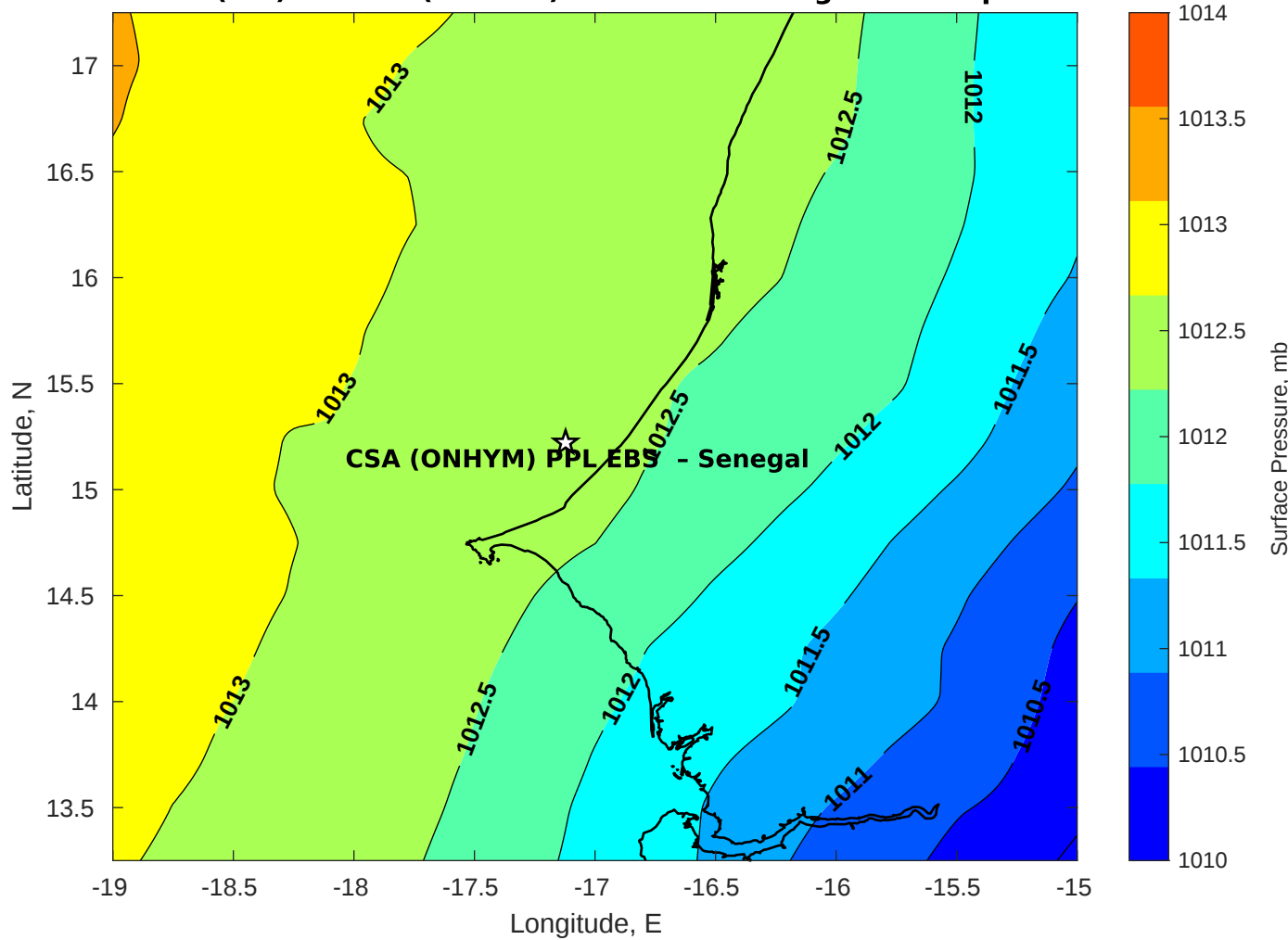
Surface Pressure (mb) for CSA (ONHYM) PPL EBS - Senegal at 11-Apr-2025 00:00:00
