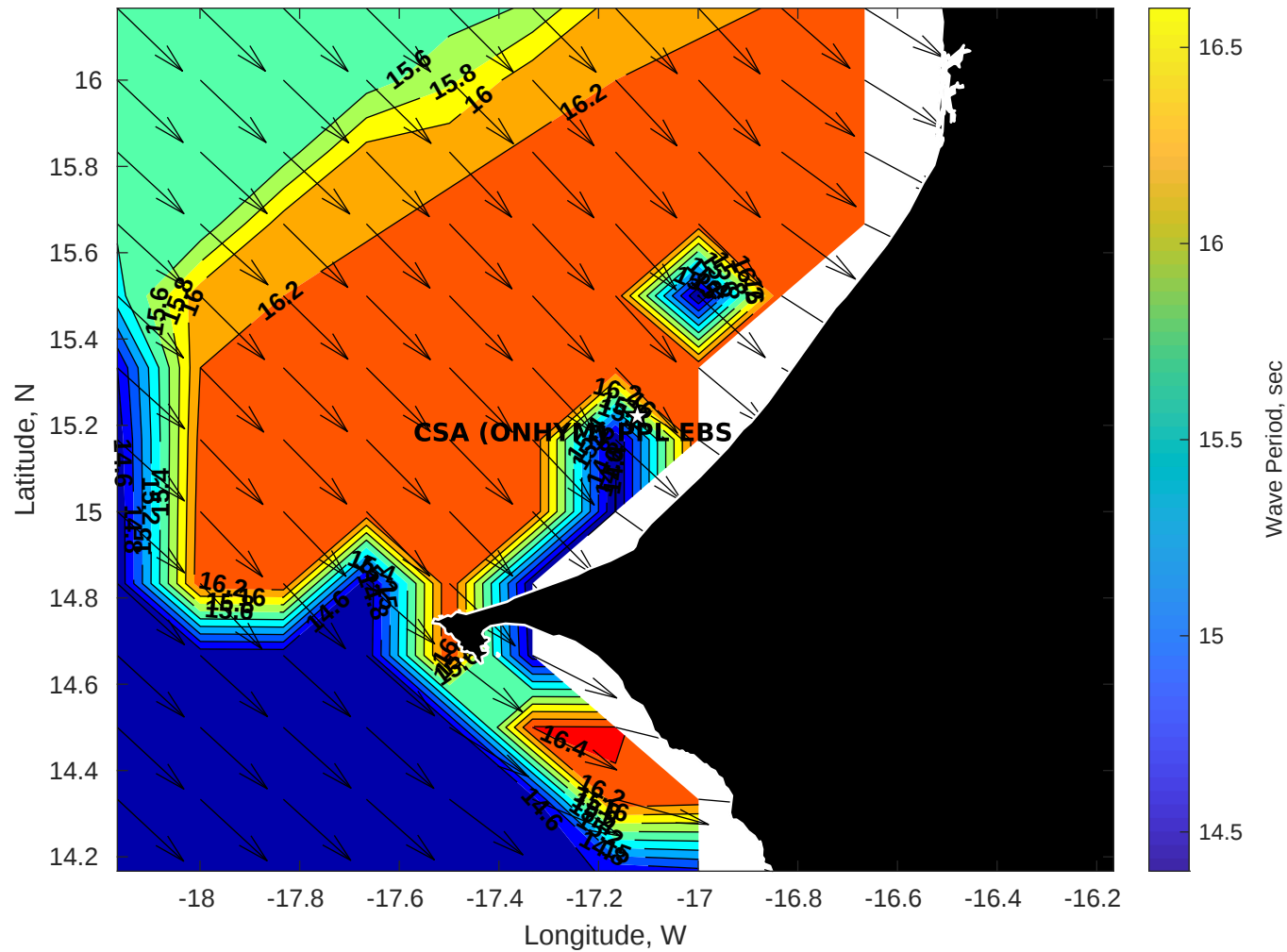
Wave Period (sec) for CSA (ONHYM) PPL EBS - Senegal at 09-Apr-2025 09:00:00
