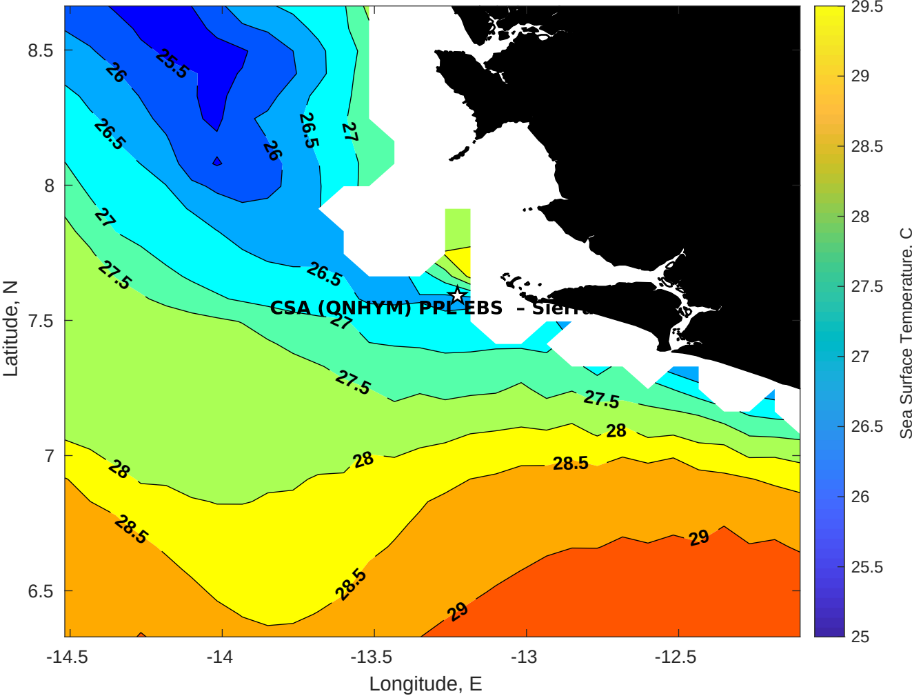
SST for CSA (ONHYM) PPL EBS - Sierra Leone at 08-Apr-2025 00:00:00
