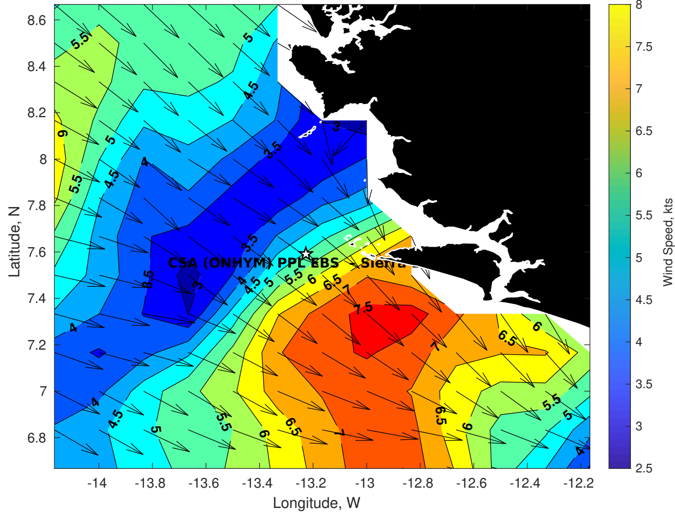
Winds (kts) for CSA (ONHYM) PPL EBS - Sierra Leone at 09-Apr-2025 09:00:00
