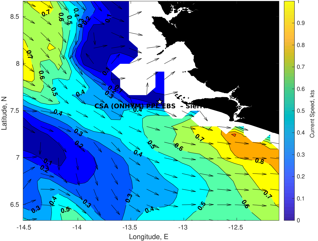
Surface Currents for CSA (ONHYM) PPL EBS - Sierra Leone at 08-Apr-2025 00:00:00
