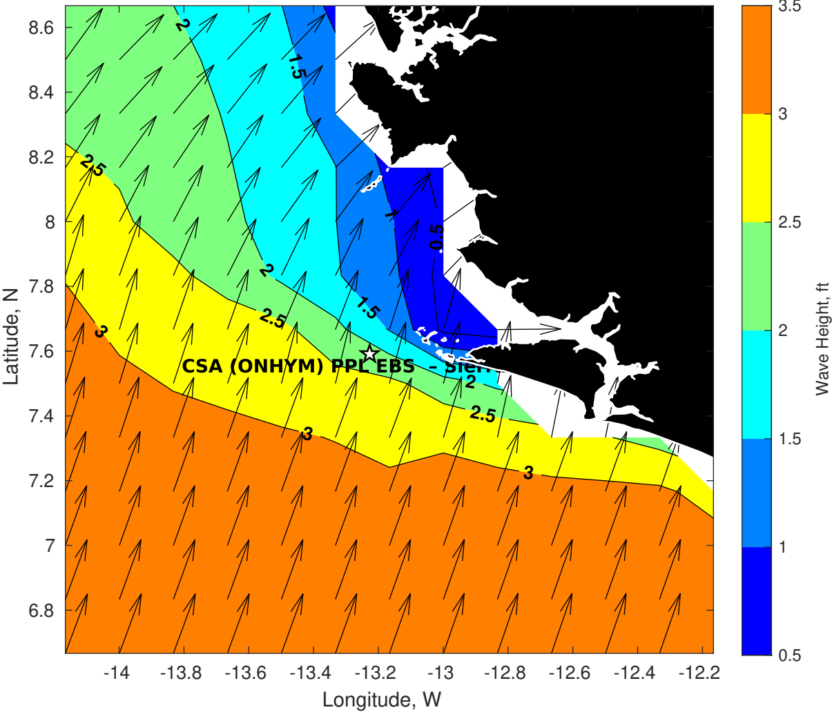
Wave Height (ft) for CSA (ONHYM) PPL EBS - Sierra Leone at 09-Apr-2025 09:00:00
