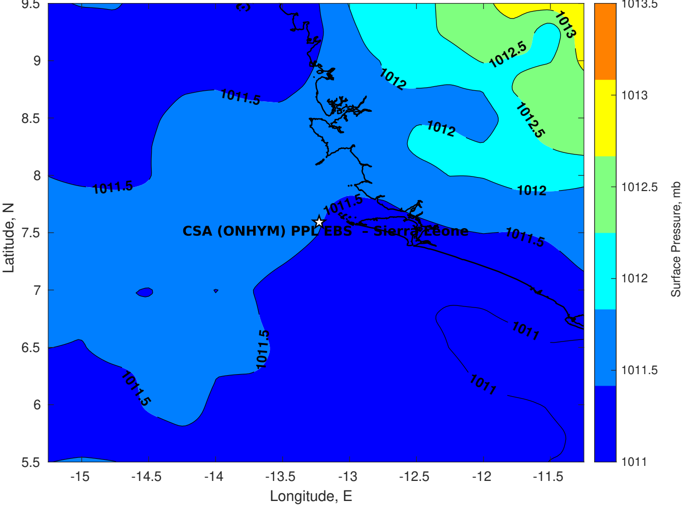
Surface Pressure (mb) for CSA (ONHYM) PPL EBS - Sierra Leone at 11-Apr-2025 00:00:00
