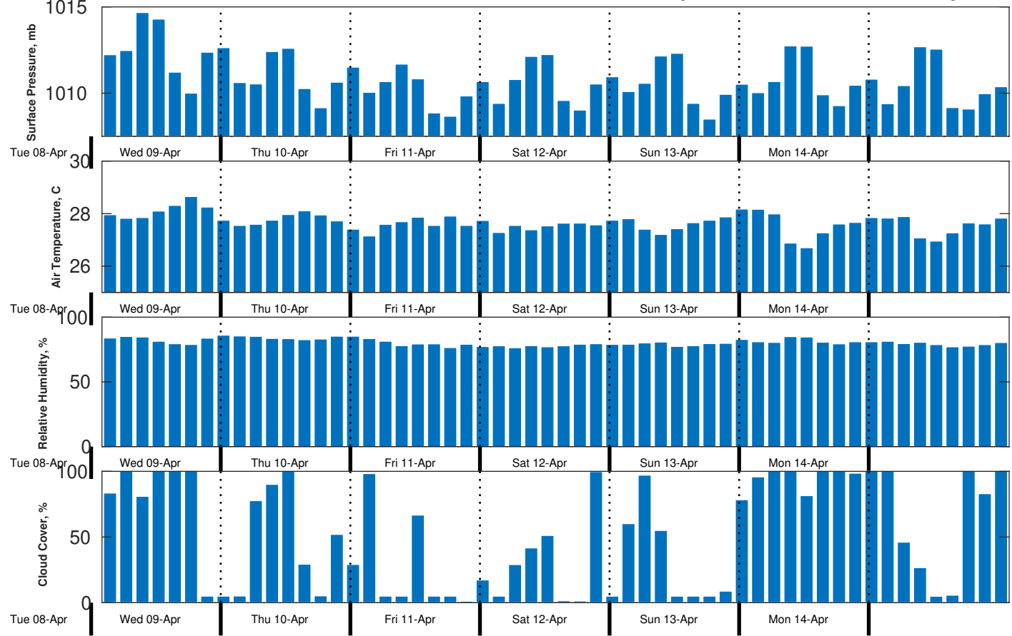
Met Forecast for CSA (ONHYM) PPL EBS - Sierra Leone from 09-Apr-2025 00:00:00 to 16-Apr-2025 00:00:00
