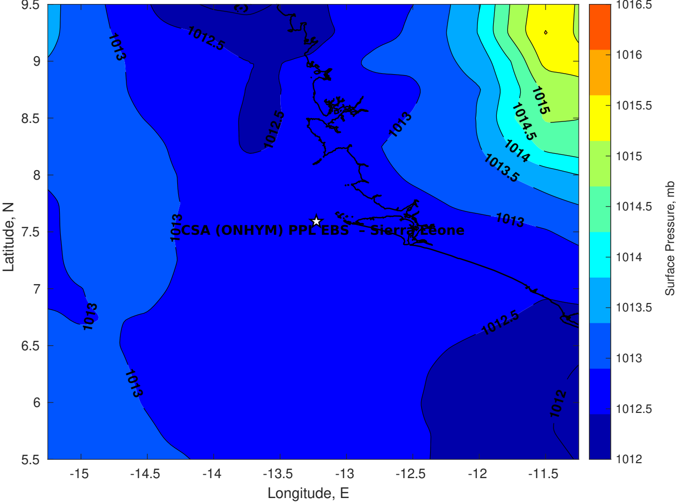
Surface Pressure (mb) for CSA (ONHYM) PPL EBS - Sierra Leone at 10-Apr-2025 00:00:00
