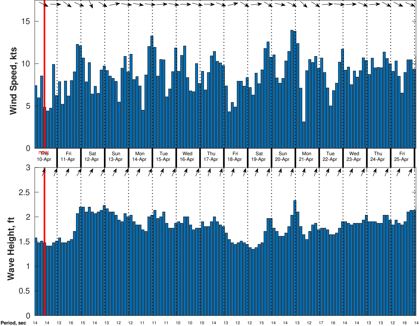
Wind & Wave Forecast for CSA (ONHYM) PPL EBS - Sierra Leone from 09-Apr-2025 01:00:00 to 25-Apr-2025 01:00:00
