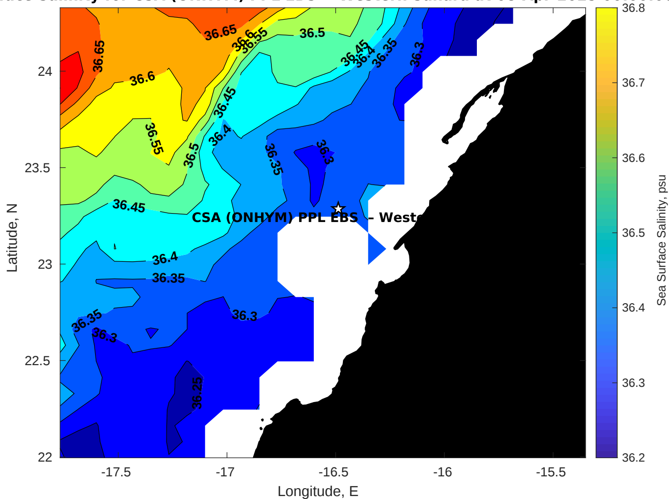
Surface Salinity for CSA (ONHYM) PPL EBS - Western Sahara at 08-Apr-2025 00:00:00
