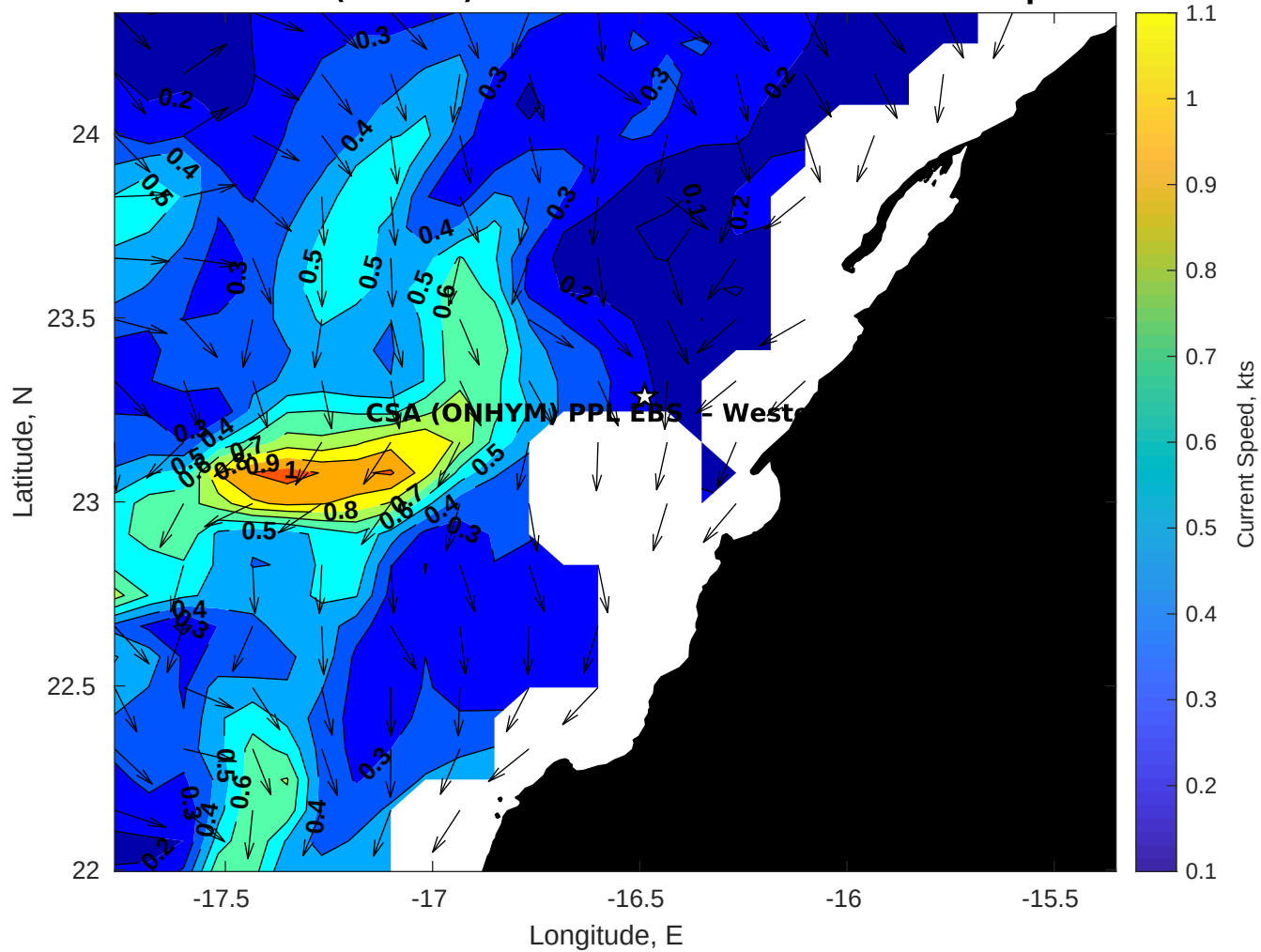
Surface Currents for CSA (ONHYM) PPL EBS - Western Sahara at 08-Apr-2025 00:00:00
