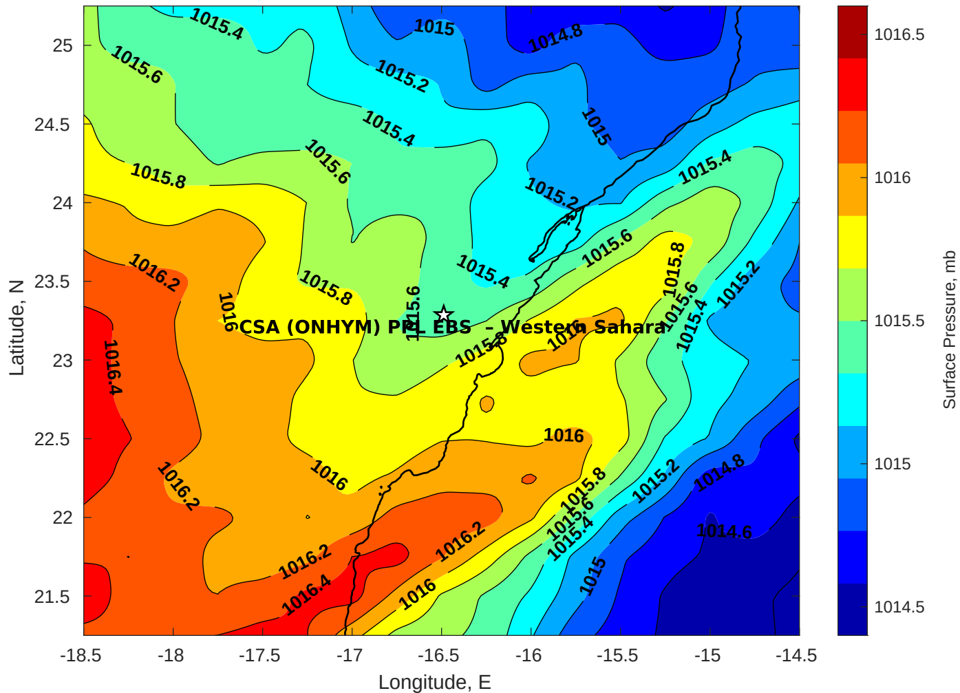
Surface Pressure (mb) for CSA (ONHYM) PPL EBS - Western Sahara at 09-Apr-2025 00:00:00
