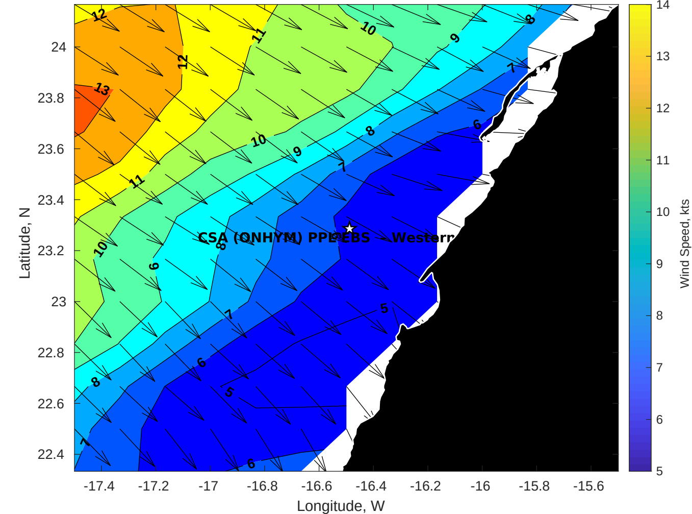
Winds (kts) for CSA (ONHYM) PPL EBS - Western Sahara at 09-Apr-2025 09:00:00
