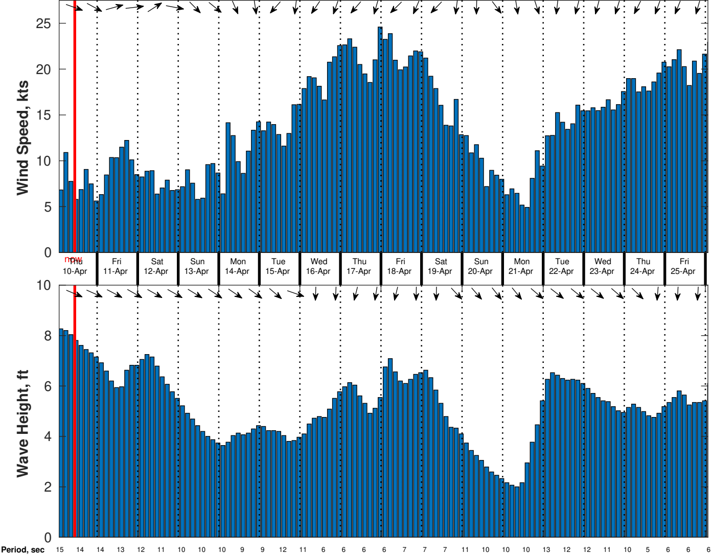
Wind & Wave Forecast for CSA (ONHYM) PPL EBS - Western Sahara from 09-Apr-2025 01:00:00 to 25-Apr-2025 01:00:00
