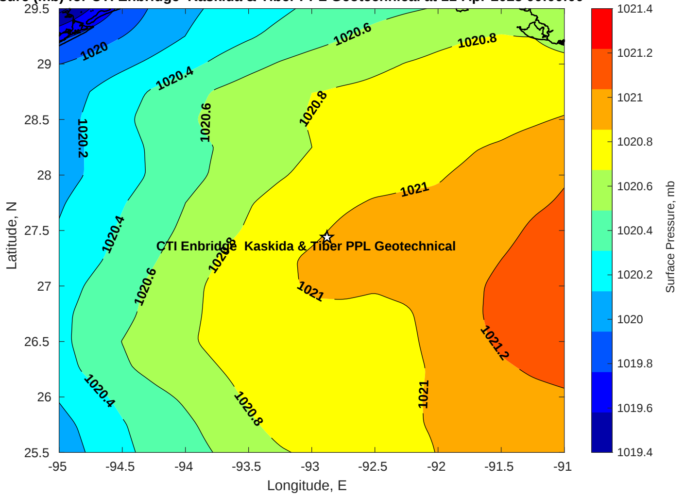
Surface Pressure (mb) for CTI Enbridge Kaskida & Tiber PPL Geotechnical at 11-Apr-2025 00:00:00
