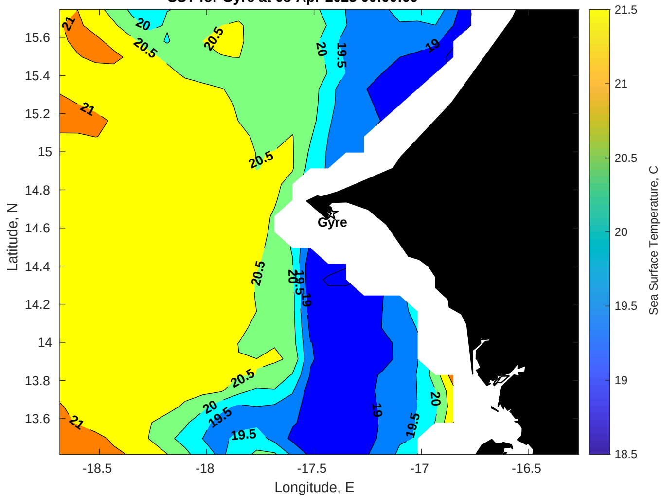
SST for Gyre at 08-Apr-2025 00:00:00
