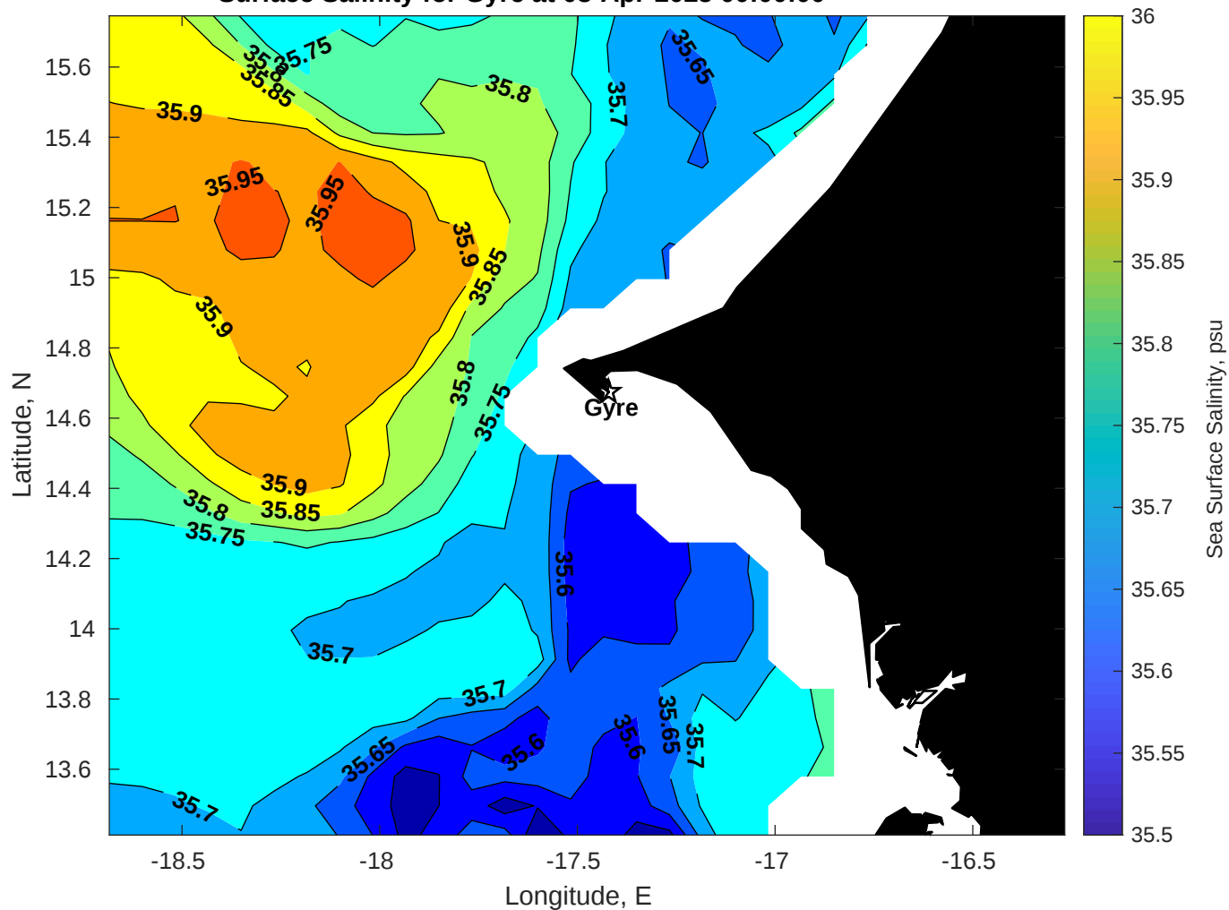
Surface Salinity for Gyre at 08-Apr-2025 00:00:00
