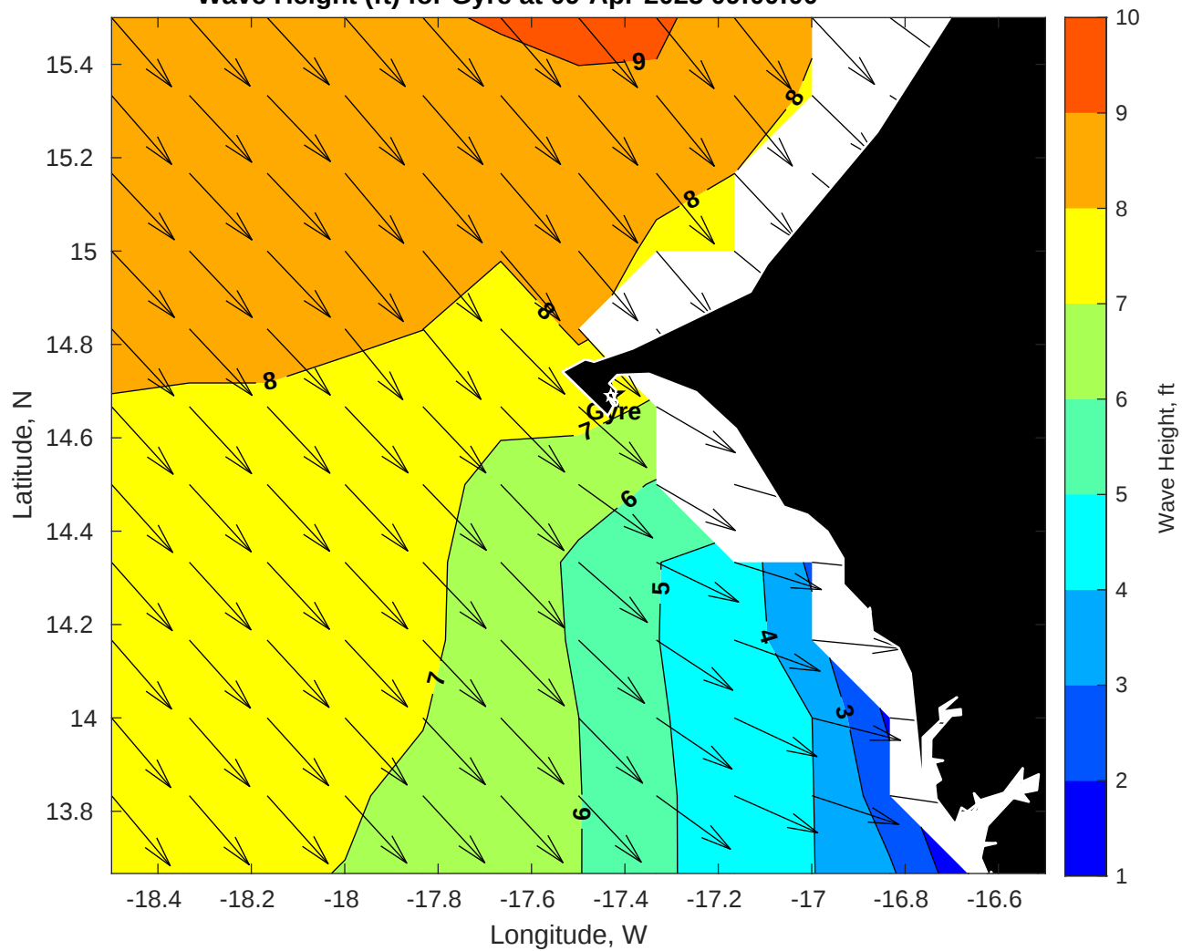
Wave Height (ft) for Gyre at 09-Apr-2025 09:00:00
