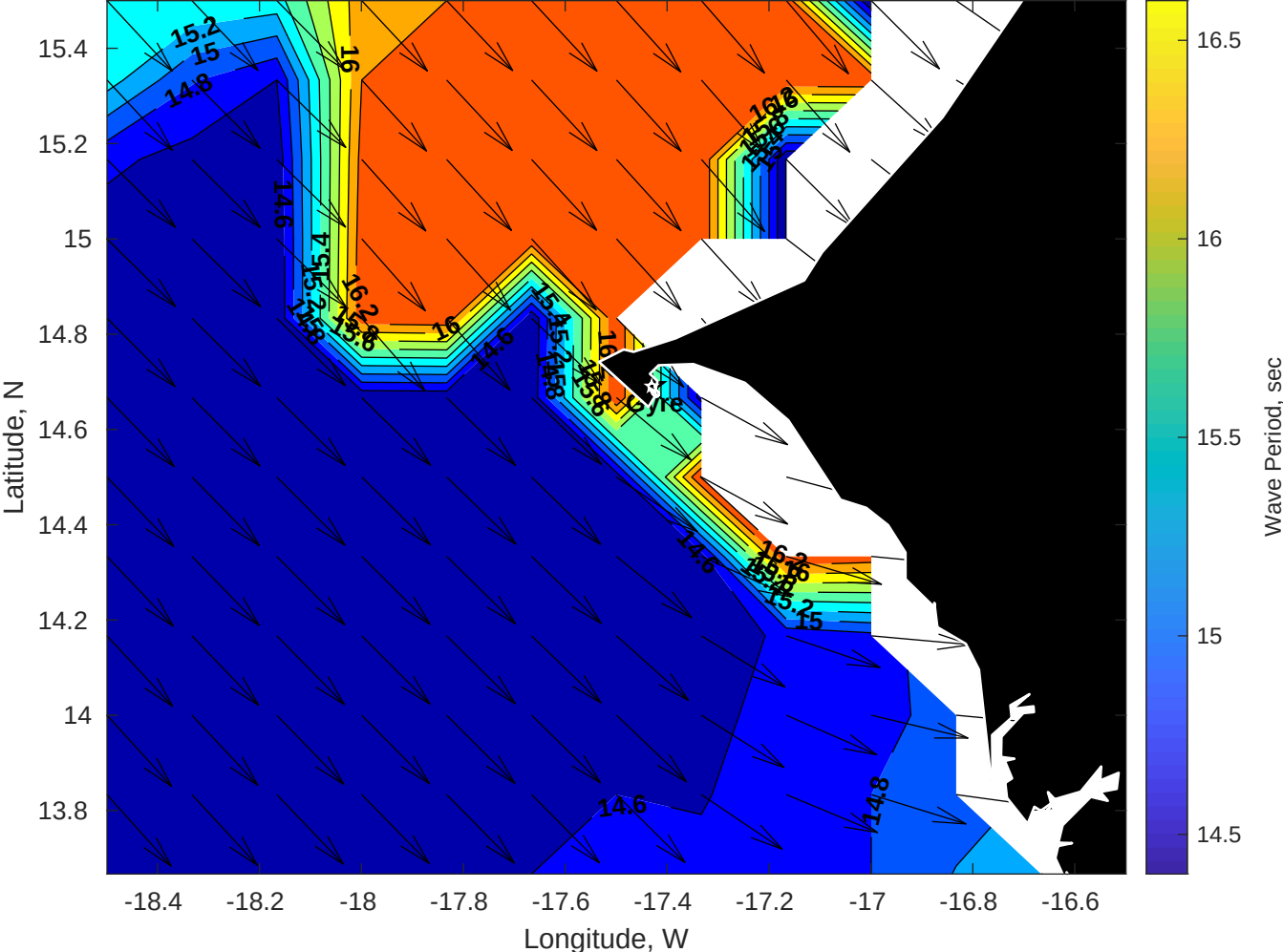
Wave Period (sec) for Gyre at 09-Apr-2025 09:00:00
